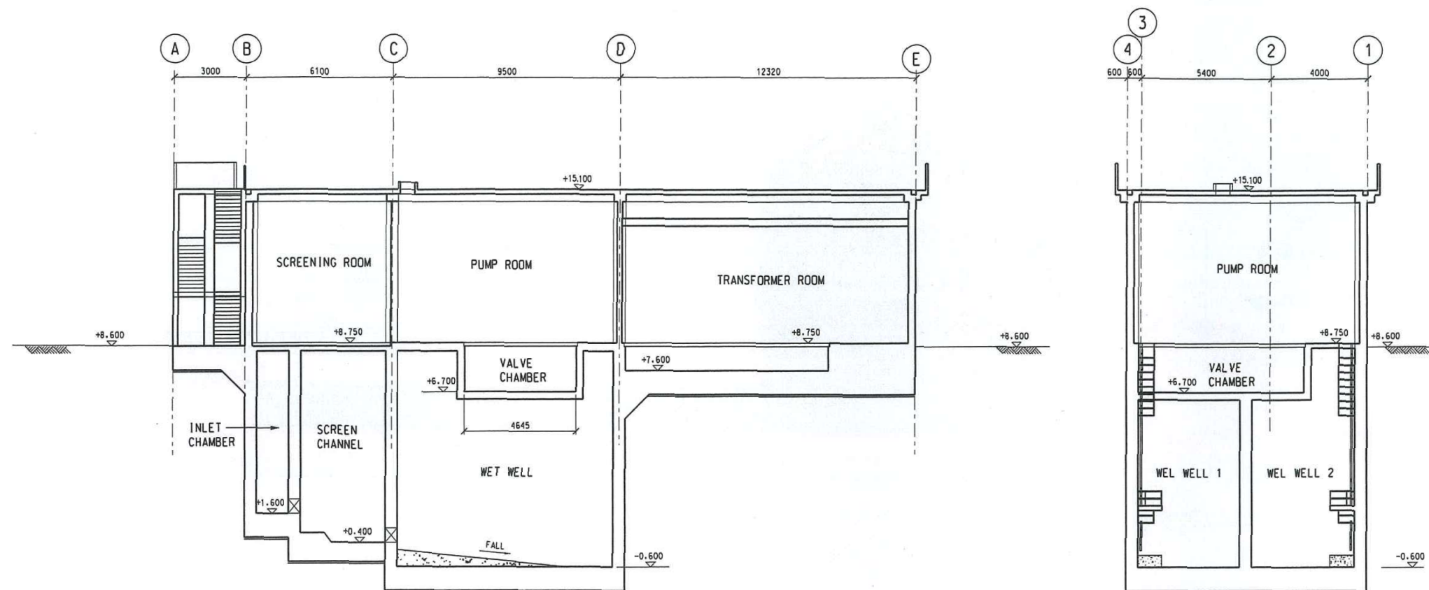
SECTION 1 SCALE 1:100 PS/001
