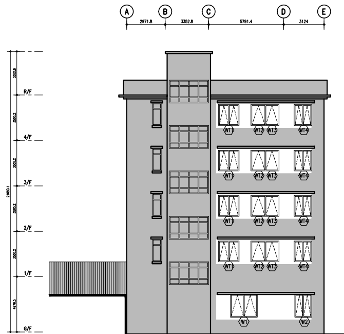
EAST ELEVATION
