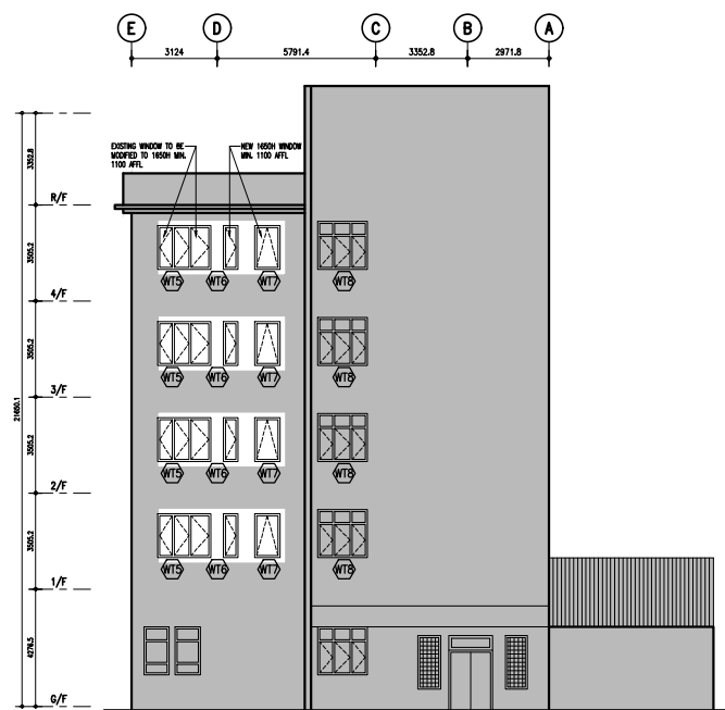
WEST ELEVATION
