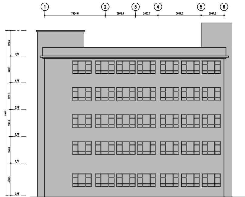
NORTH ELEVATION
