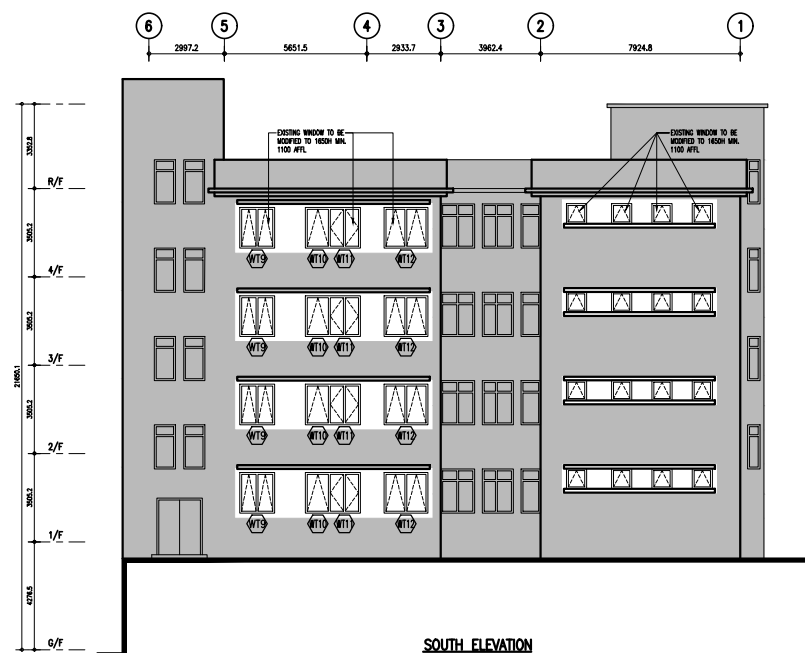
SOUTH ELEVATION
