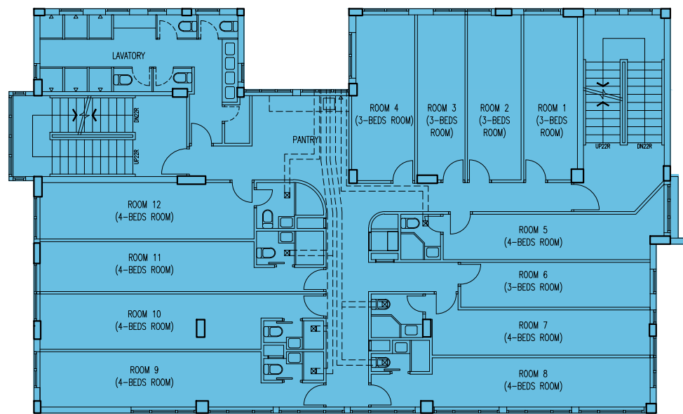
TYPICAL (2/F TO 4/F) FLOOR PLAN
