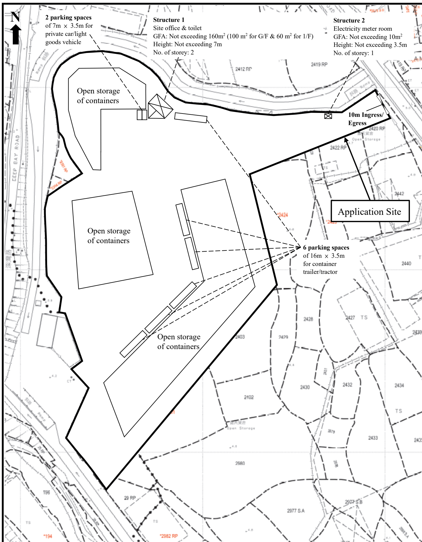
Figure 3: Proposed Layout Plan (Revised on 2.6.2025)
