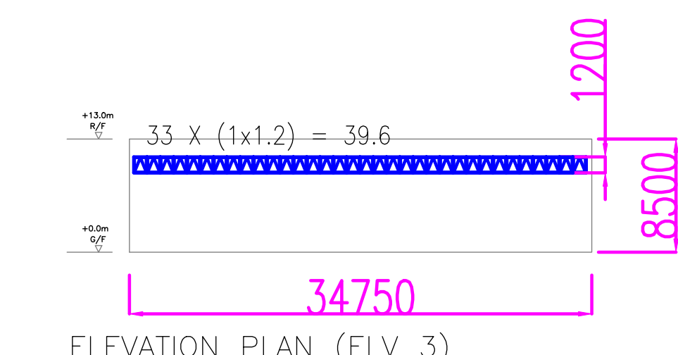
ELEVATION PLAN (ELV 3)
