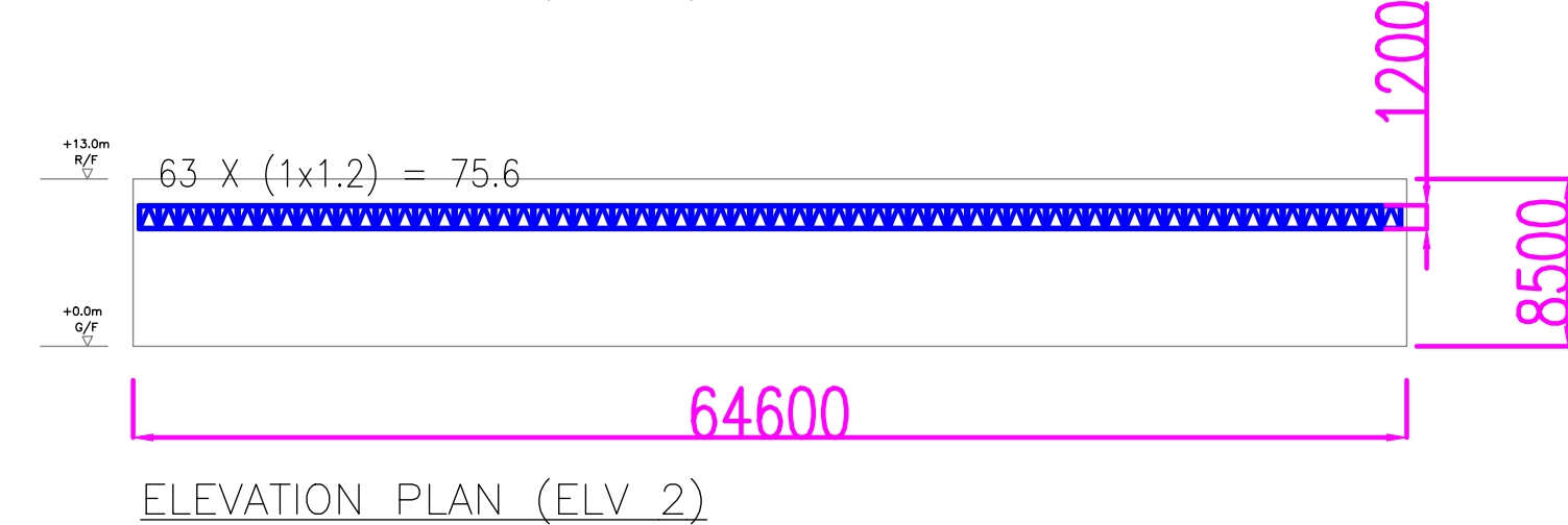
ELEVATION PLAN (ELV 2)
