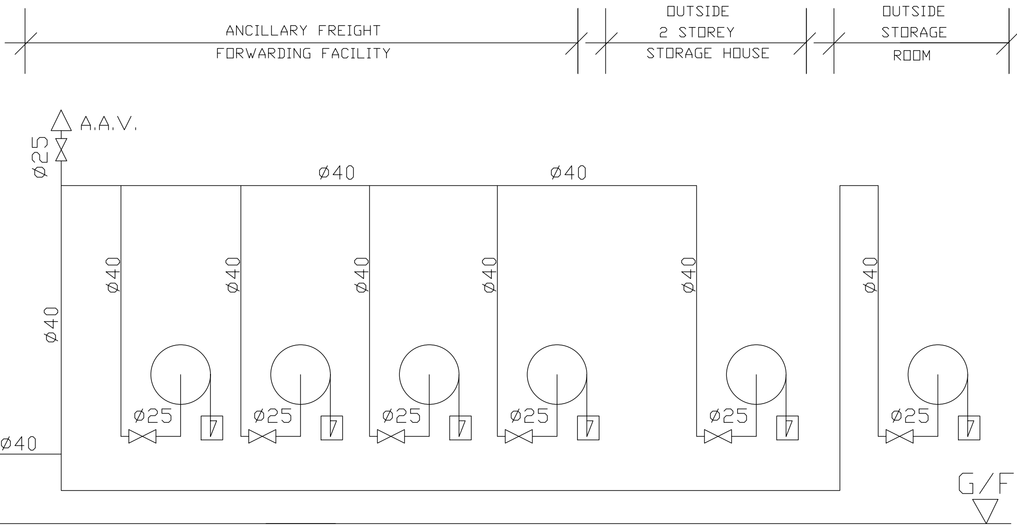
SCHEMATIC DIAGRAM FOR HOSE REEL SYSTEM
