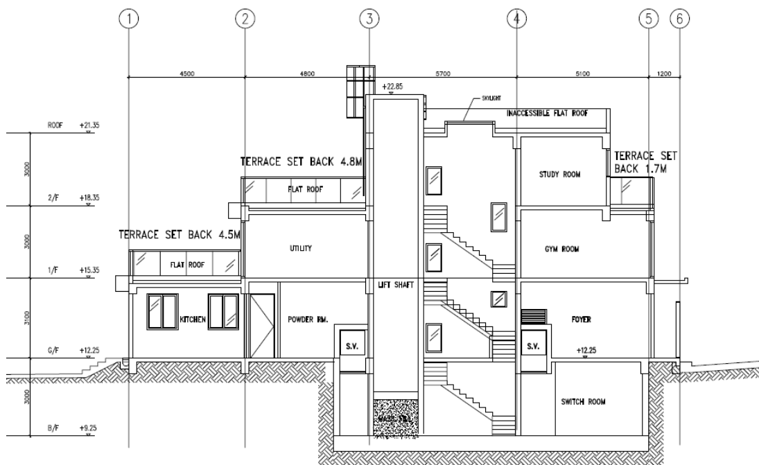
Plan 5 Section Plan of the Proposed Scheme
