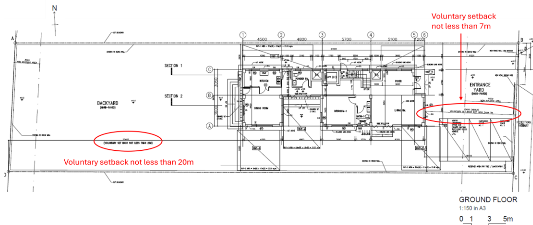
Plan 4 G/F Plan of the Proposed Scheme
