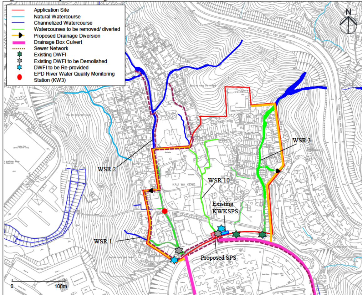
Figure 10.3: Proposed Drainage Diversion and Sewer Network
