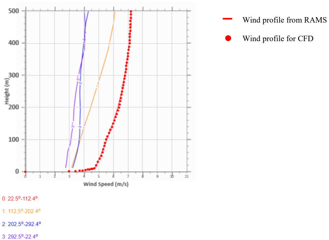
Figure 20 Vertical Wind Profile of 22.5° – 112.4° Winds
