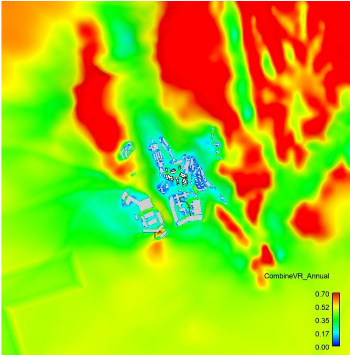
Figure C 107 Annual Weighted Average Domain Contour Plot of VR
