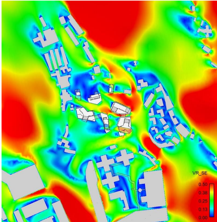
Figure C 29 Contour Plot of VR under SE Wind
