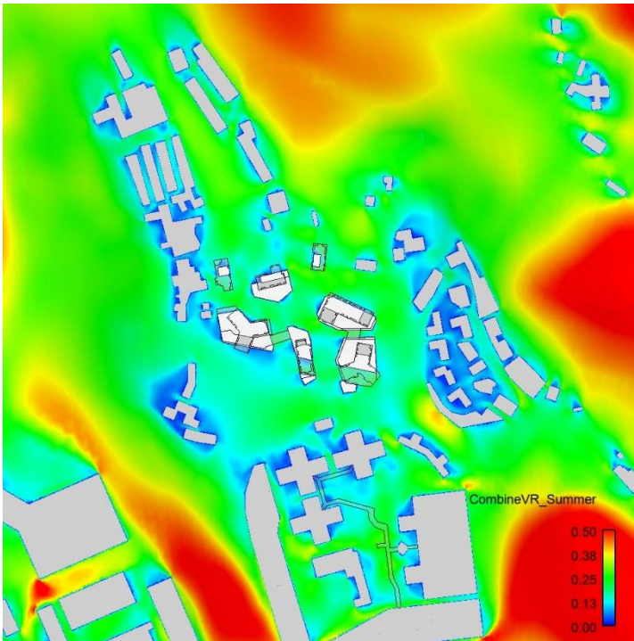
Figure C 36 Summer Weighted Average Contour Plot of VR
