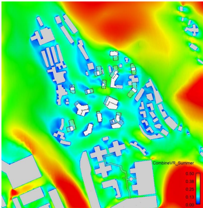
Figure C 48 Summer Weighted Average Contour Plot of VR
