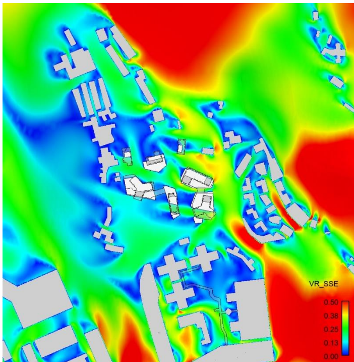
Figure C 30 Contour Plot of VR under SSE Wind
