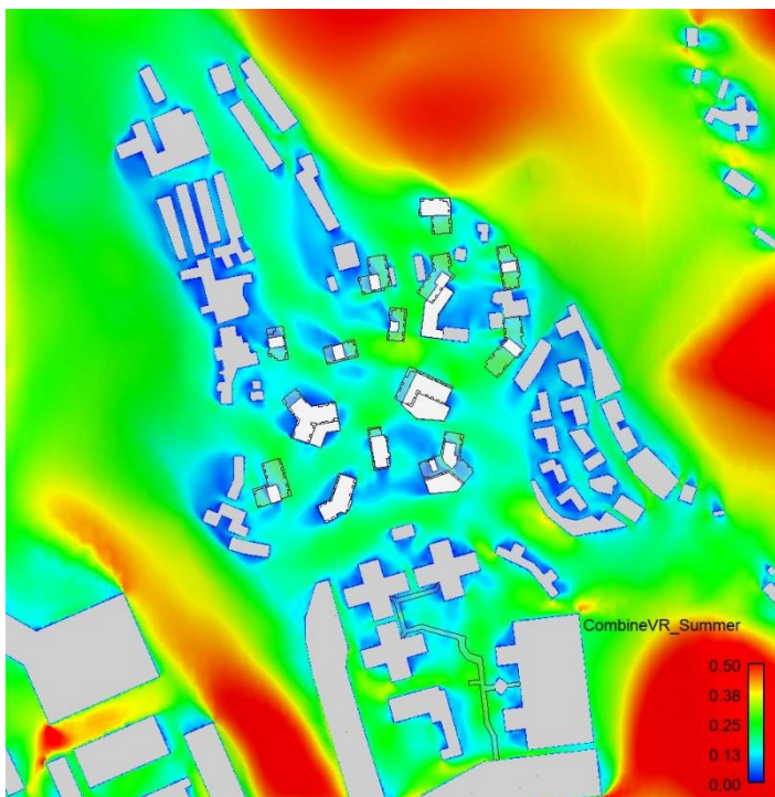
Figure C 12 Summer Weighted Average Contour Plot of VR
