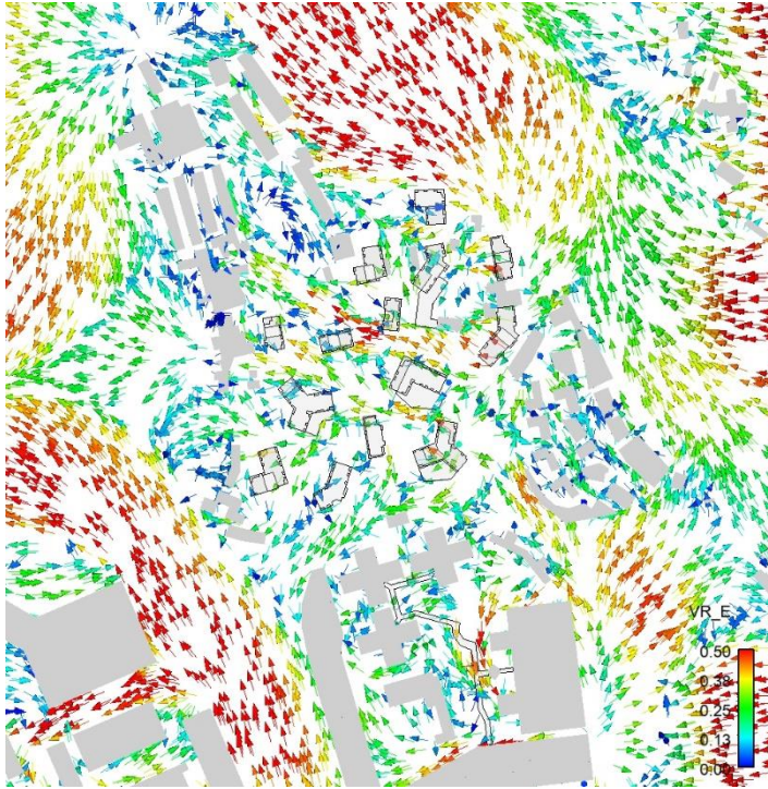
Figure D 3 Vector Plot of VR under E Wind
