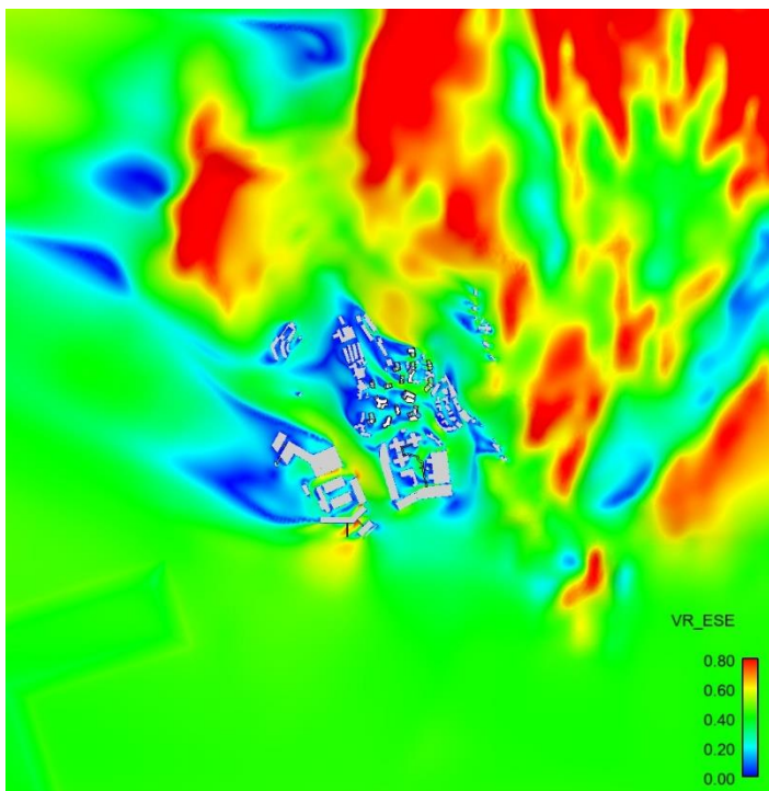
Figure C 76 Domain Contour Plot of VR under ESE Wind
