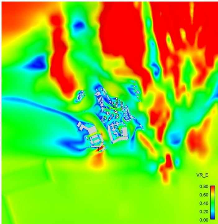
Figure C 75 Domain Contour Plot of VR under E Wind
