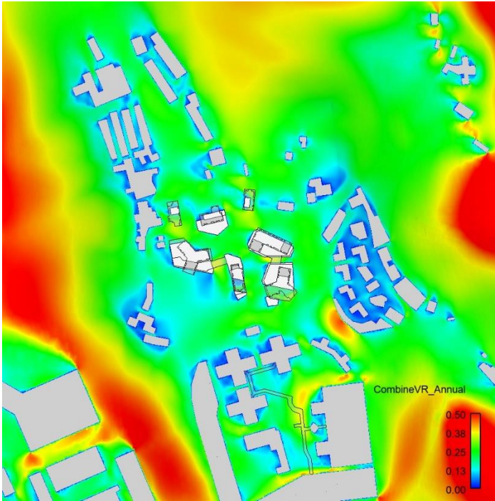
Figure C 35 Annual Weighted Average Contour Plot of VR
