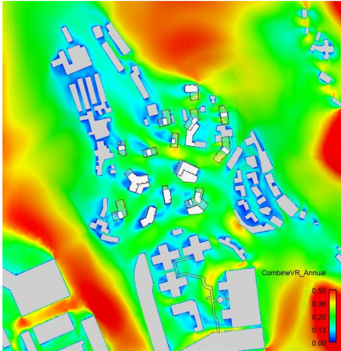
Figure C 47 Annual Weighted Average Contour Plot of VR
