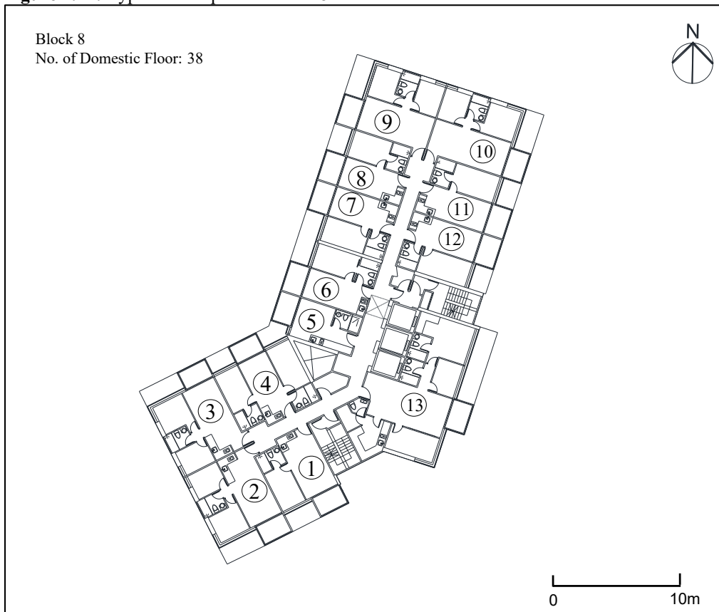
Figure 2.14: Typical floor plan of Block 8
