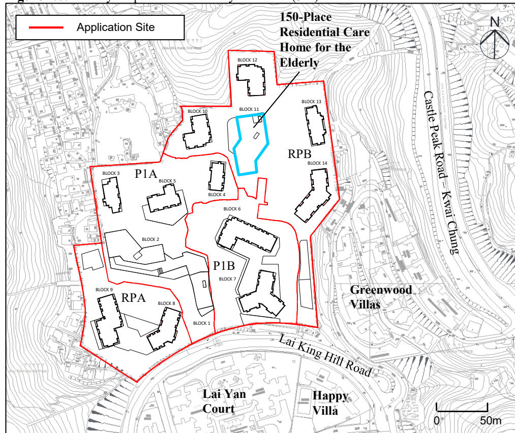
Figure 2.6: Site layout plan – Community Facilities (3/F)
