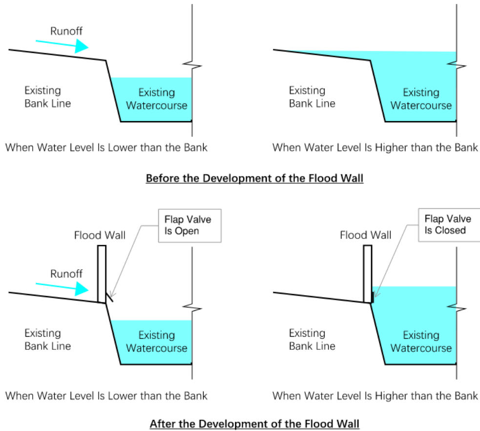
Figure 5.2 – Illustration of the Surface Runoff Before and After the Development of the Flood Wall
