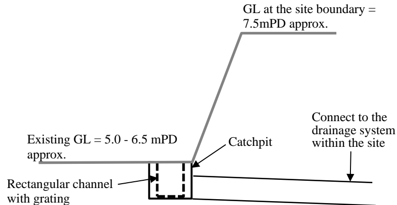
Figure 5.1 – Typical Section of the Proposed Rectangular Channel
