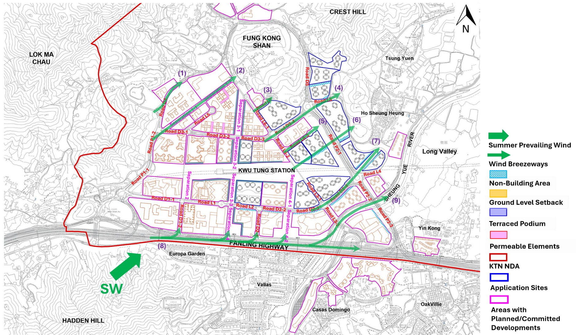
Figure C2.5(a) Wind Flow under the SW Summer Prevailing Wind for the OZP Compliant Scheme
