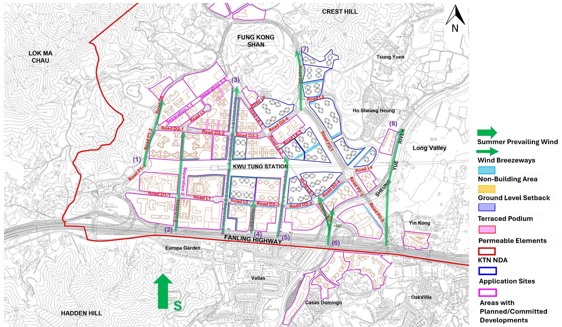
Figure C2.4(a) Wind Flow under the S Summer Prevailing Wind for the OZP Compliant Scheme
