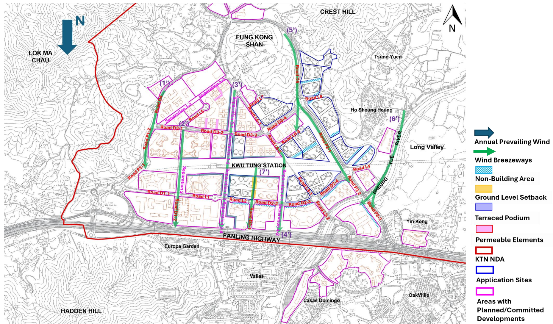
Figure C2.1(b) Wind Flow under the N Annual Prevailing Wind for the Proposed Scheme
