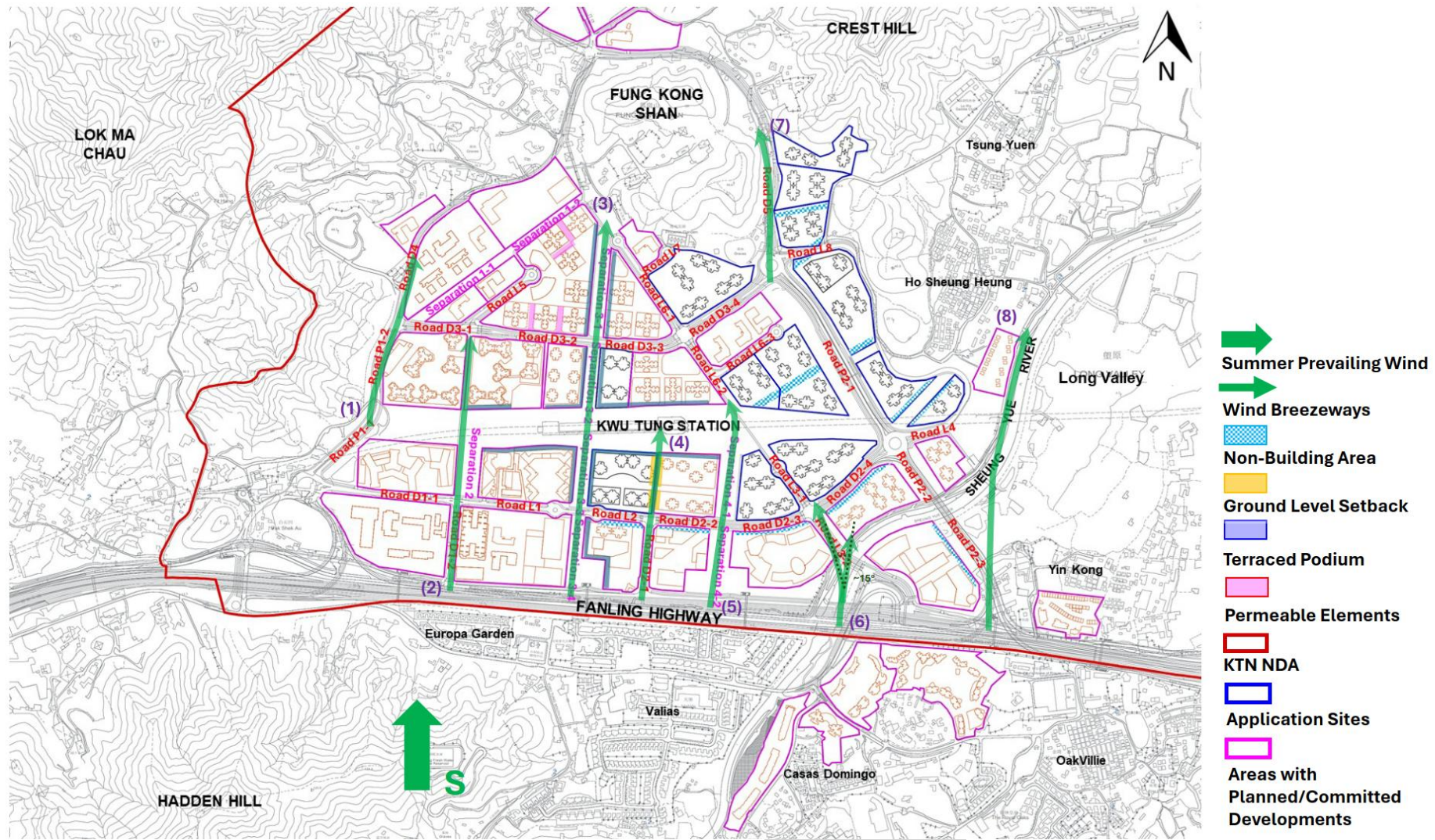
Figure 8.4(a) Wind Flow under the S Summer Prevailing Wind for the Approved Scheme
