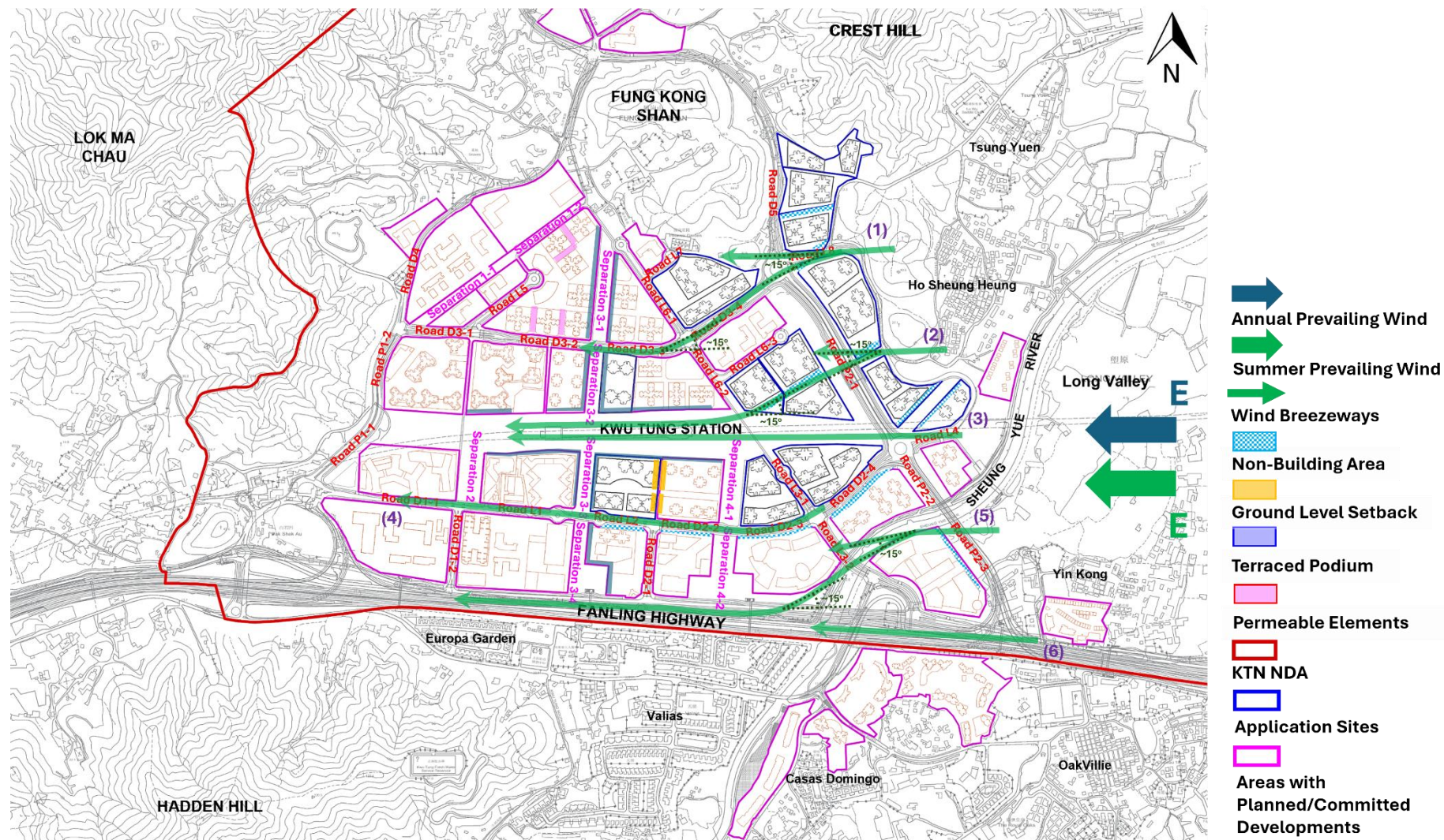
Figure 8.3(b) Wind Flow under the E Annual and Summer Prevailing Wind for the Proposed Scheme
