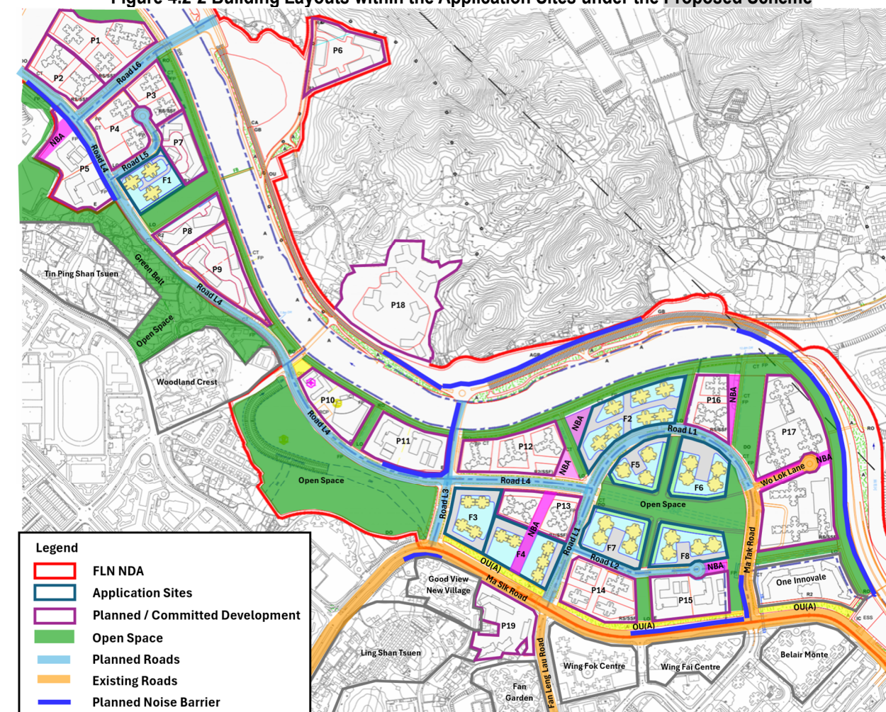
Figure 4.2-2 Building Layouts within the Application Sites under the Proposed Scheme
