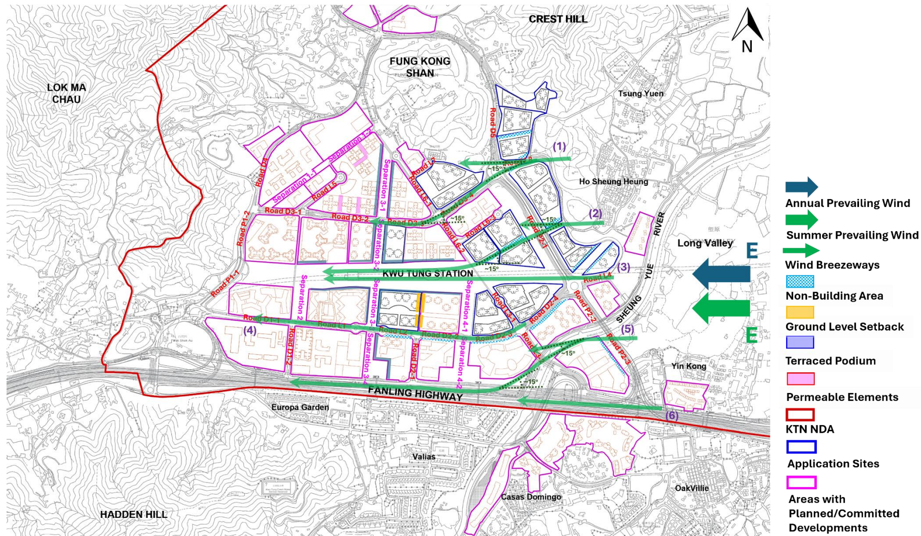
Figure C2.3(b) Wind Flow under the E Annual and Summer Prevailing Wind for the Proposed Scheme
