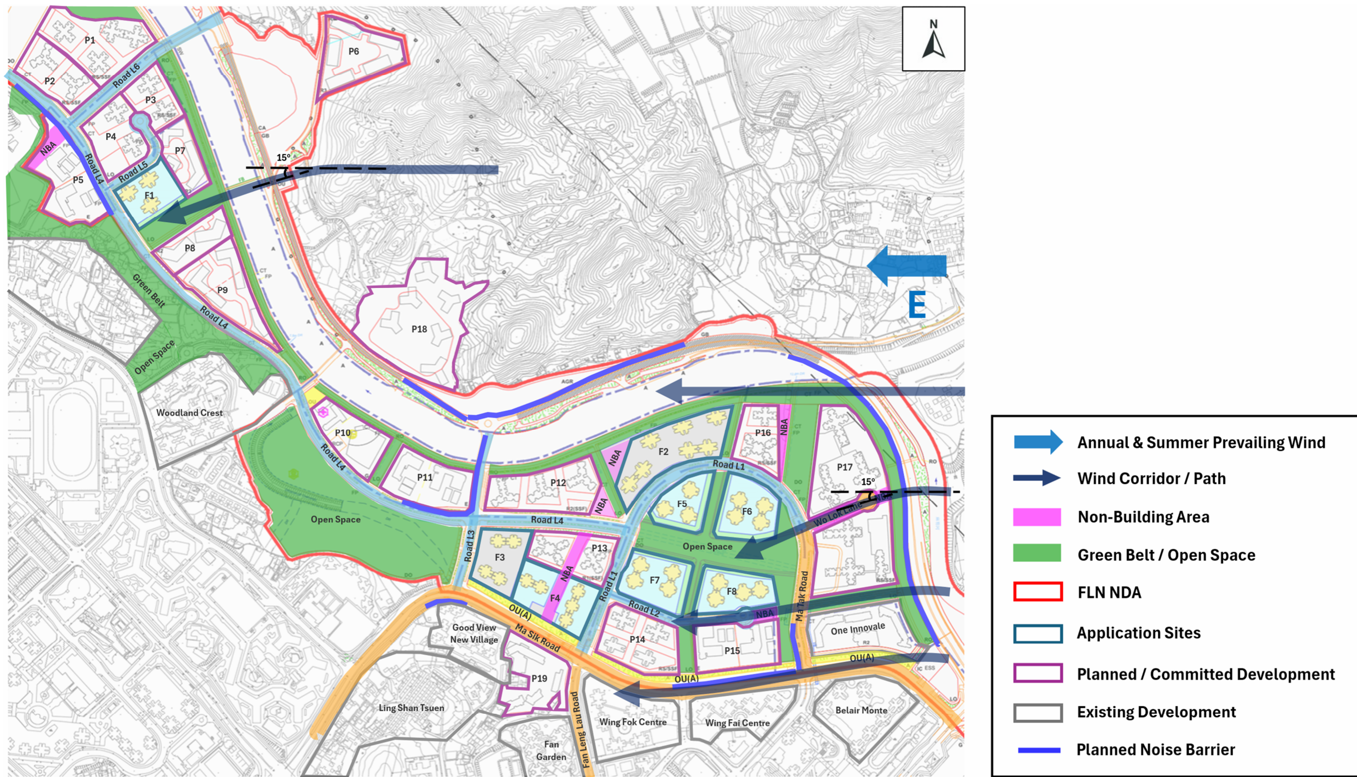
Figure 5.4-1 Wind Flow under the E Annual and Summer Prevailing Wind for the Approved Scheme
