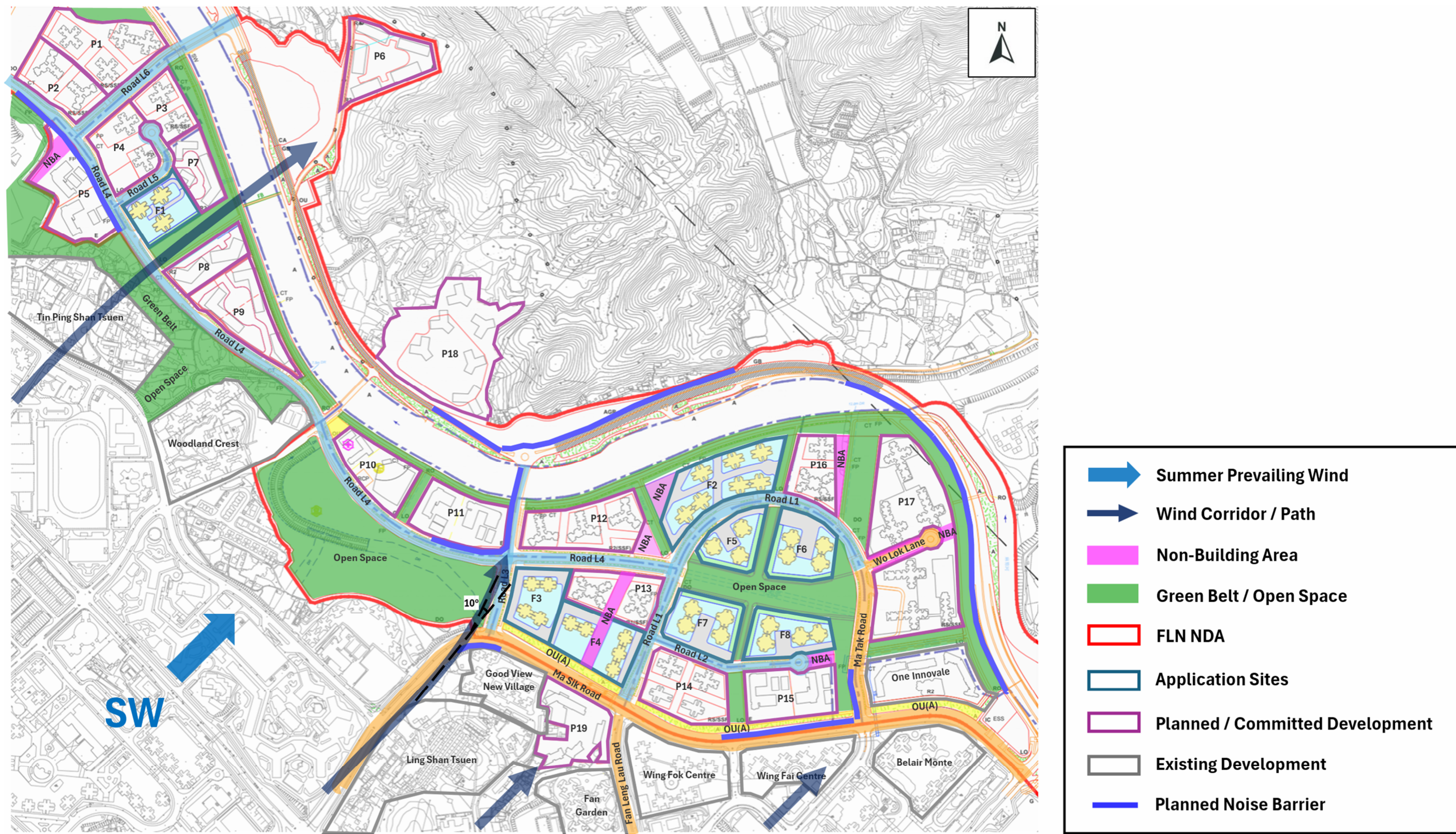
Figure 5.4-8 Wind Flow under the SW Summer Prevailing Wind for the Proposed Scheme
