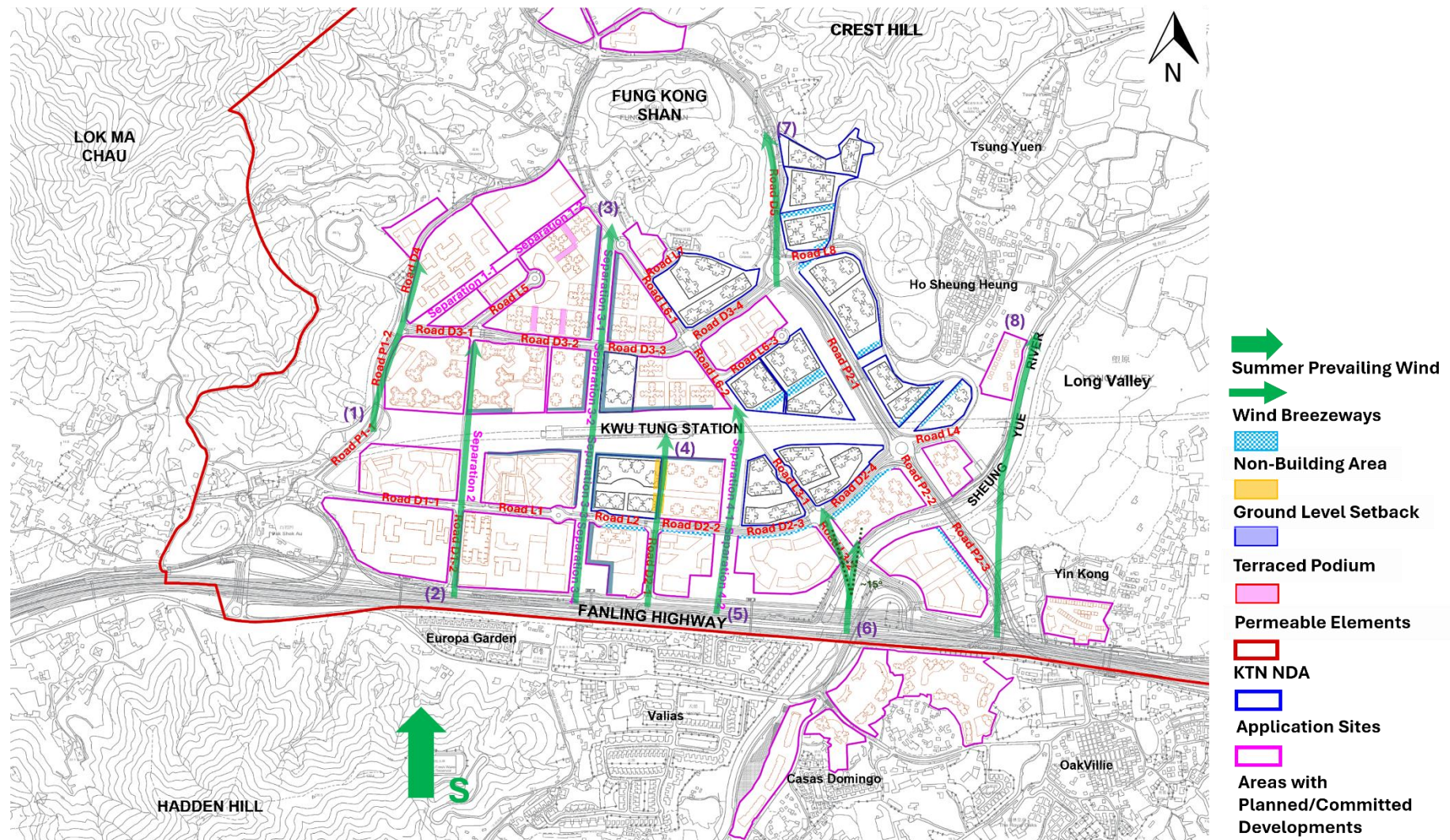
Figure 8.4(b) Wind Flow under the S Summer Prevailing Wind for the Proposed Scheme
