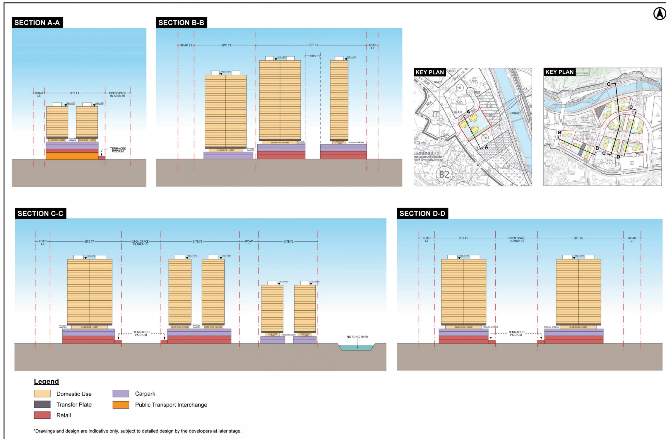
Figure 4.2-3 Indicative Sections Drawing of Application Sites under the Proposed Scheme
