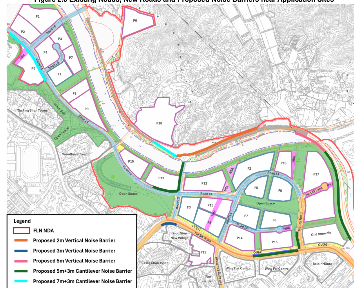
Figure 2.5 Existing Roads, New Roads and Proposed Noise Barriers near Application Sites
