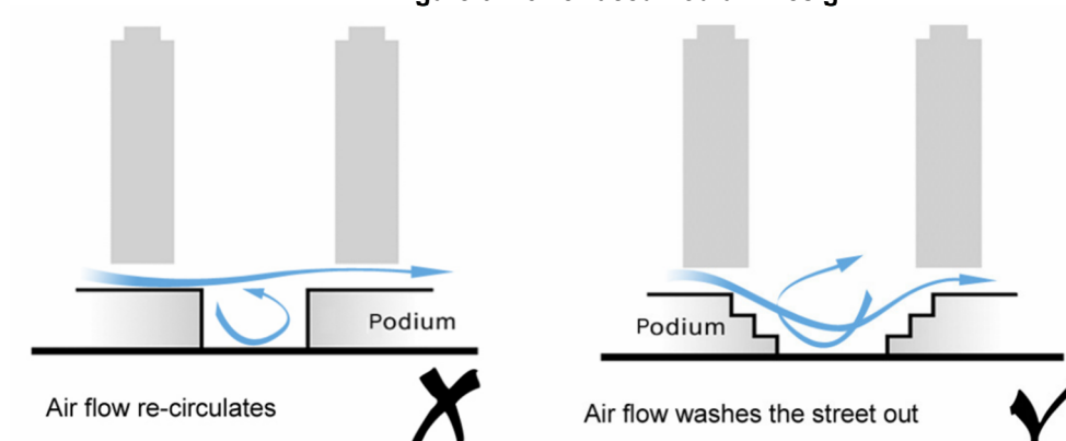
Figure 6.1-3 Terraced Podium Design
