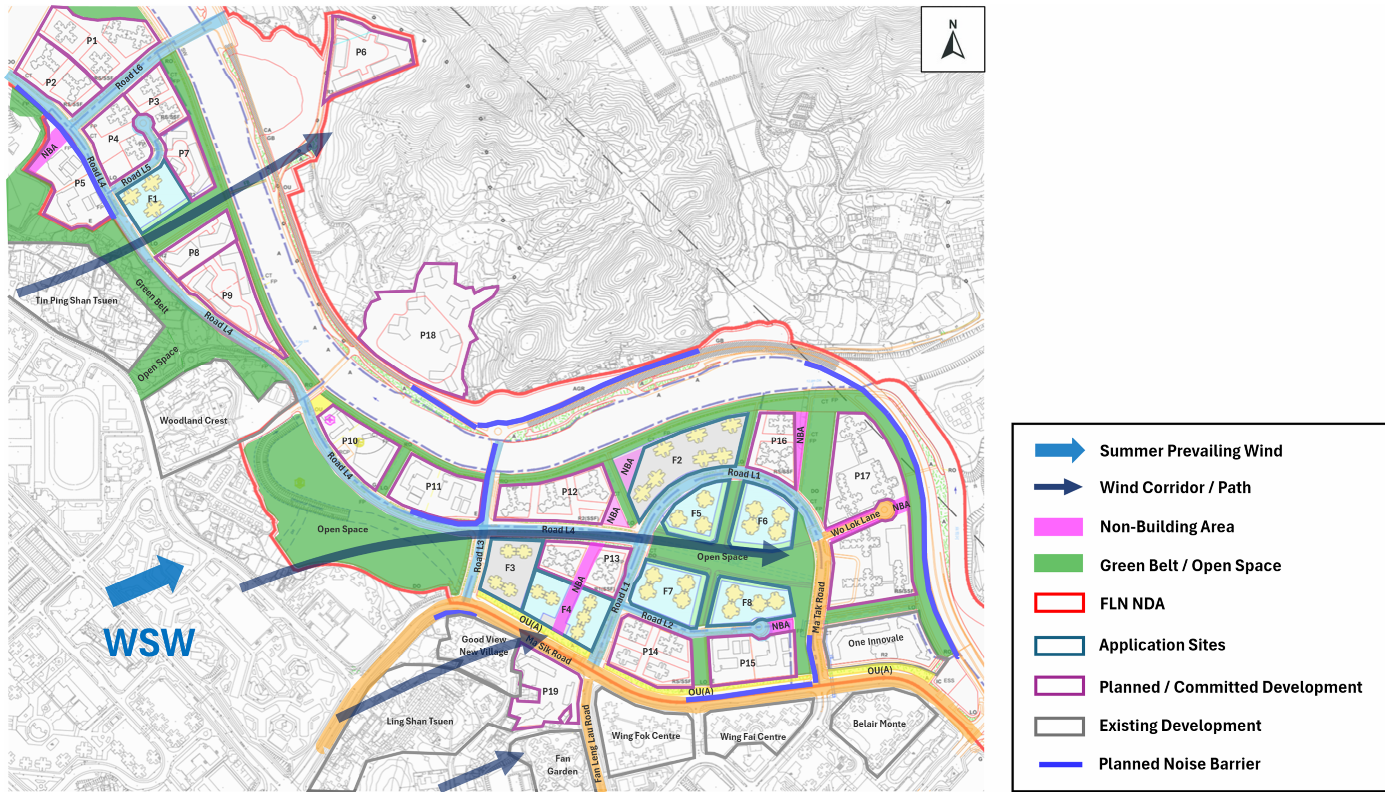
Figure 5.4-9 Wind Flow under the WSW Summer Prevailing Wind for the Approved Scheme
