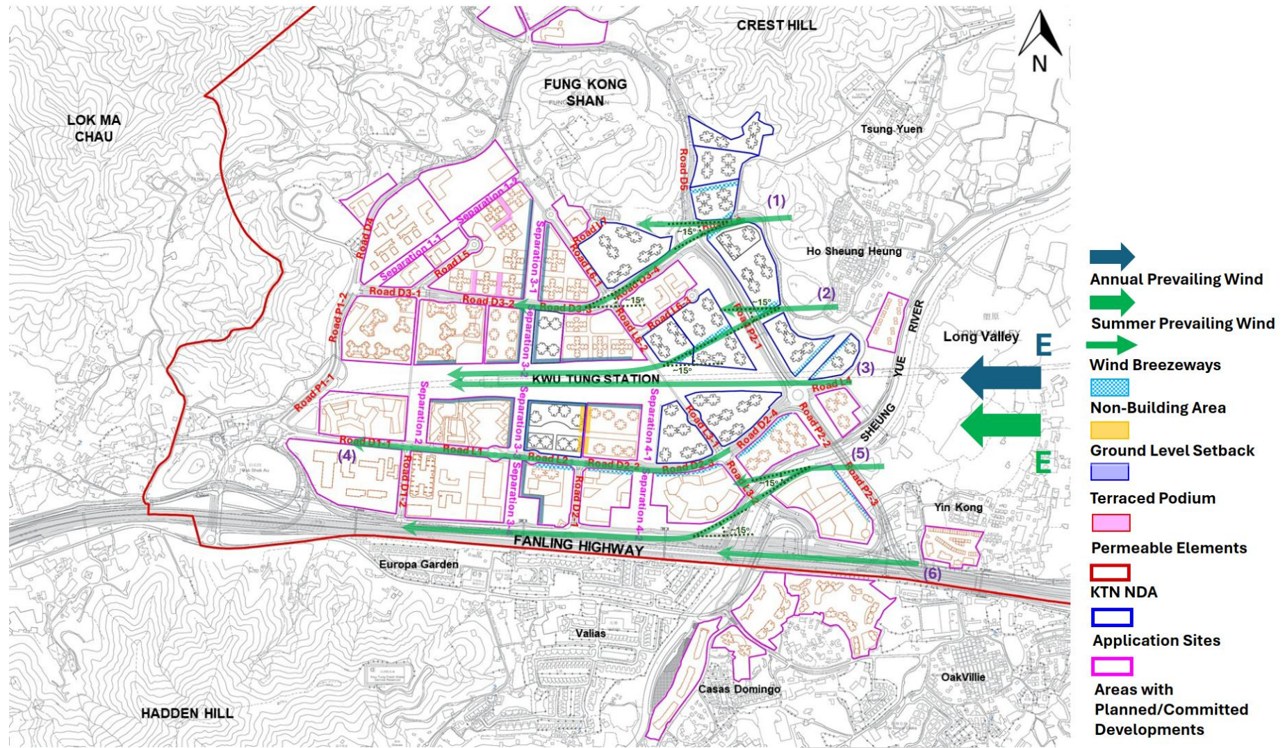
Figure 8.3(a) Wind Flow under the E Annual and Summer Prevailing Wind for the Approved Scheme
