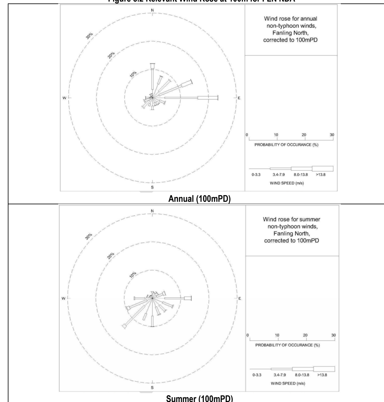
Figure 3.2 Relevant Wind Rose at 100m for FLN NDA
