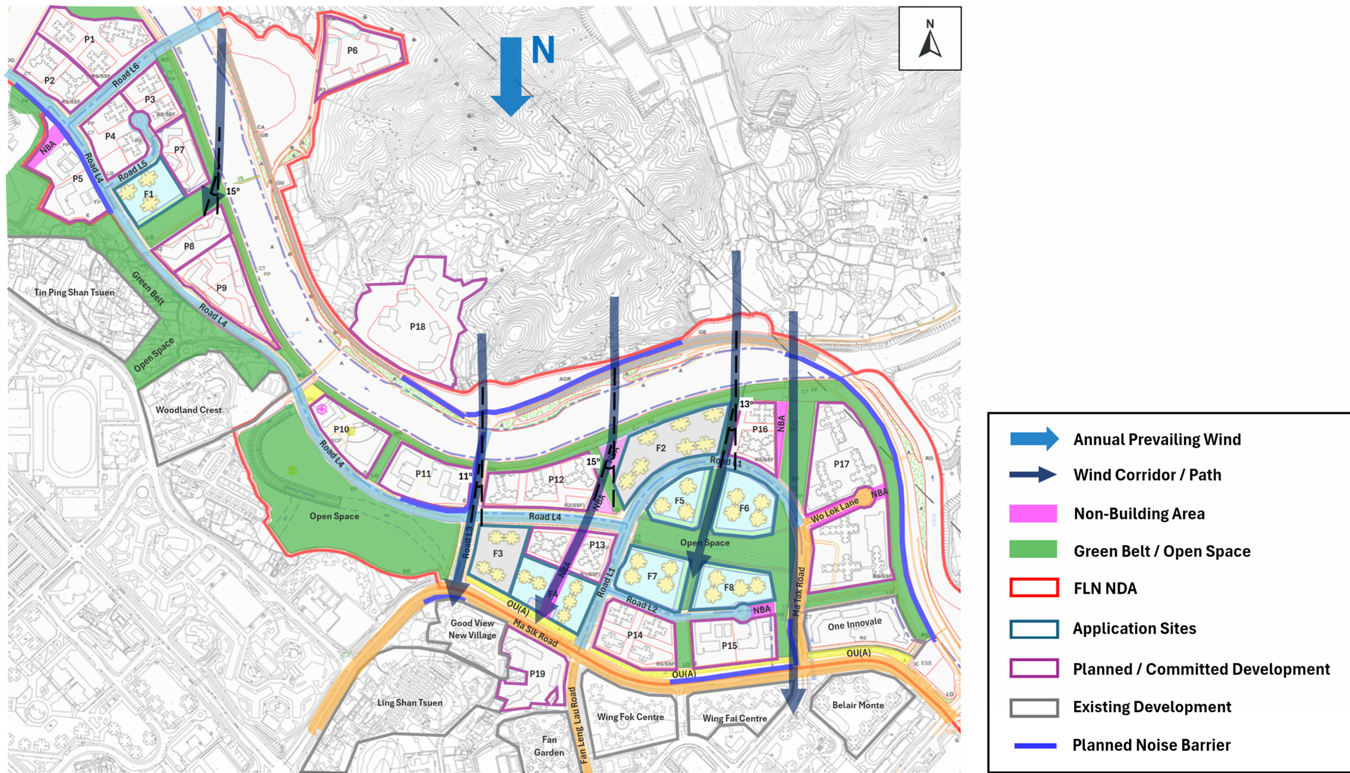
Figure 5.4-5 Wind Flow under the N Annual Prevailing Wind for the Approved Scheme
