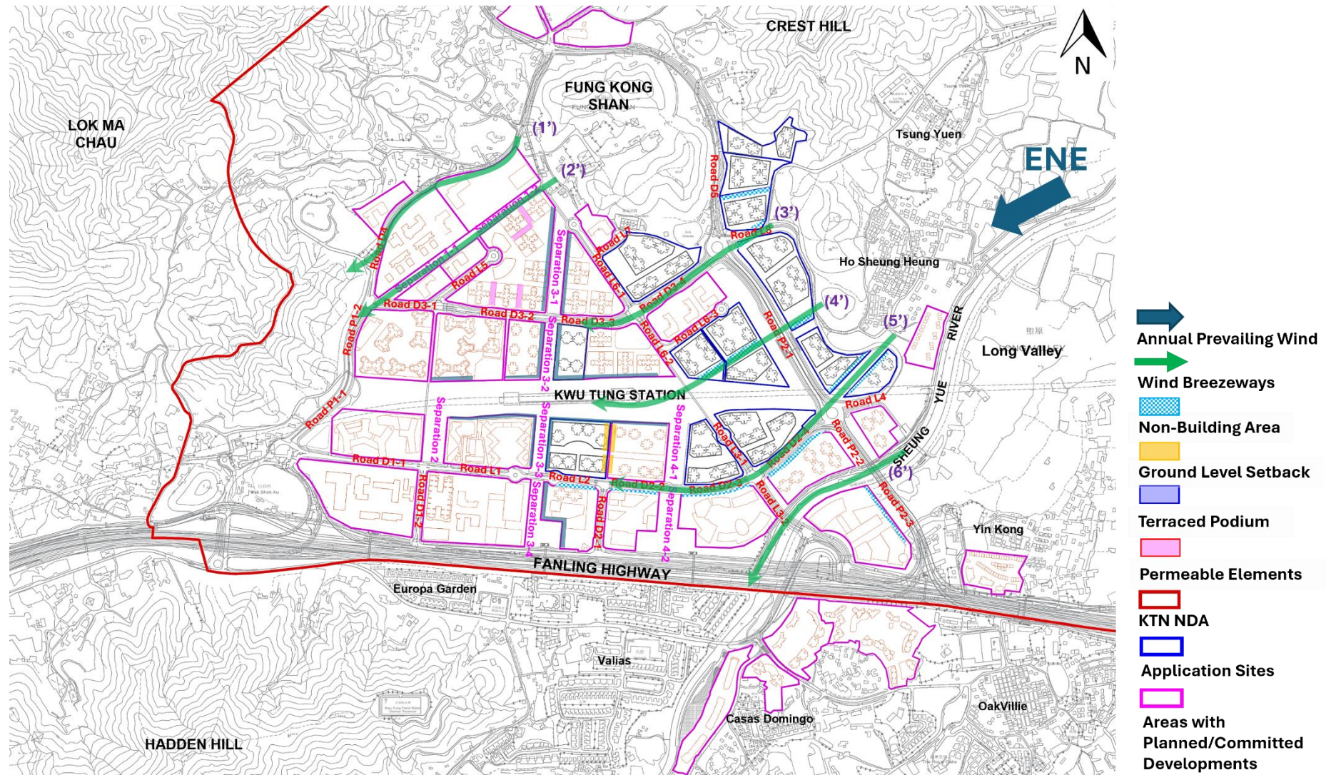
Figure C2.2(b) Wind Flow under the ENE Annual Prevailing Wind for the Proposed Scheme
