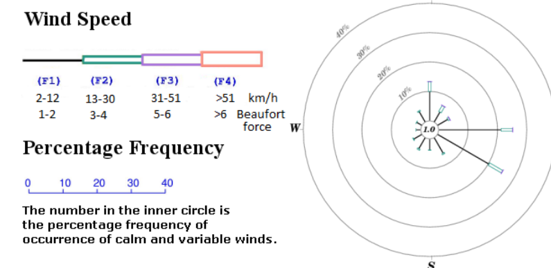
Figure 3.1-3 Summer Wind Rose from Ta Kwu Ling Weather Station Jun – Aug (1986 – 2024)
