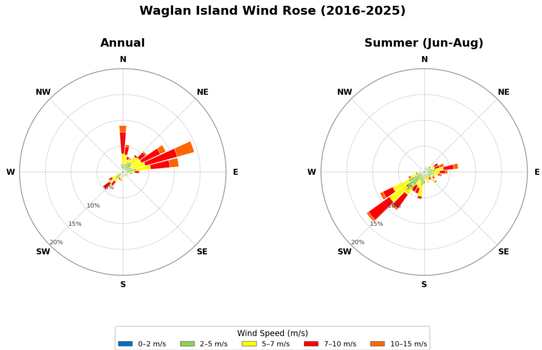
Figure 5.7 Wind Roses recorded at Waglan Island Weather Station (2016-2025)
