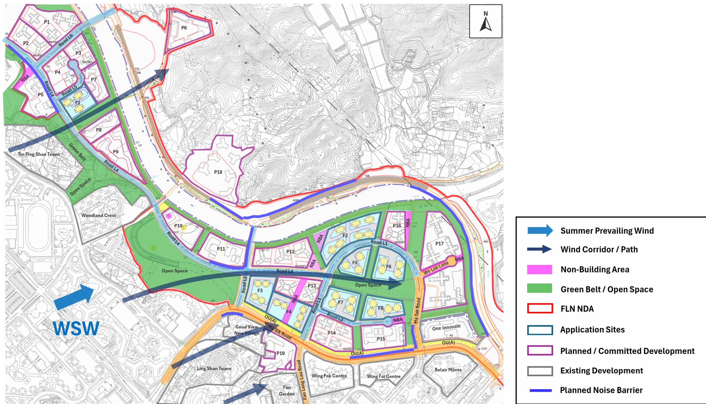
Figure 5.4-10 Wind Flow under the WSW Summer Prevailing Wind for the Proposed Scheme
