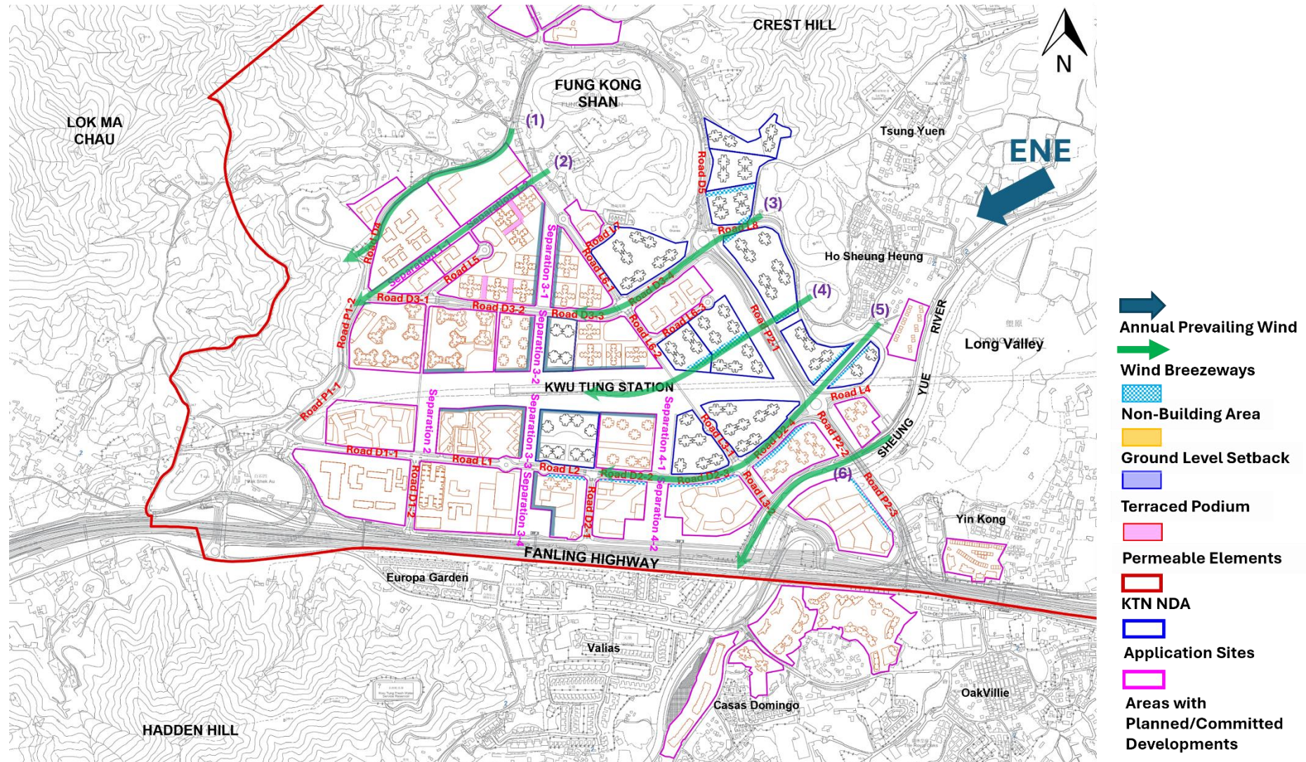
Figure C2.2(a) Wind Flow under the ENE Annual Prevailing Wind for the OZP Compliant Scheme
