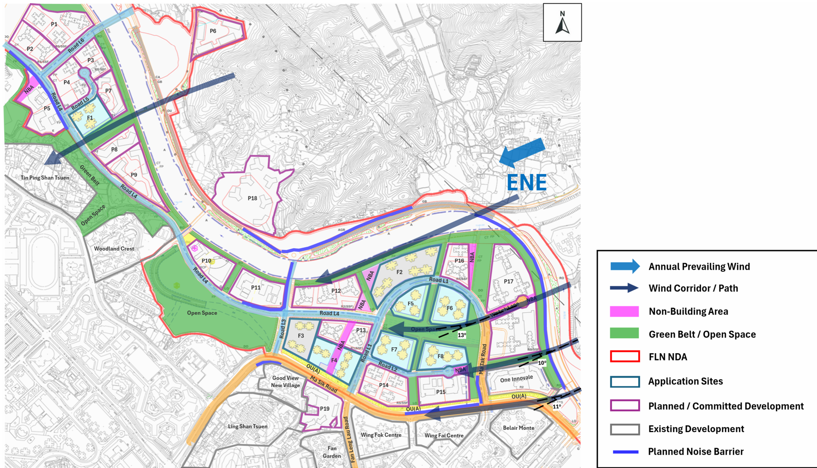
Figure 5.4-3 Wind Flow under the ENE Annual Prevailing Wind for the Approved Scheme
