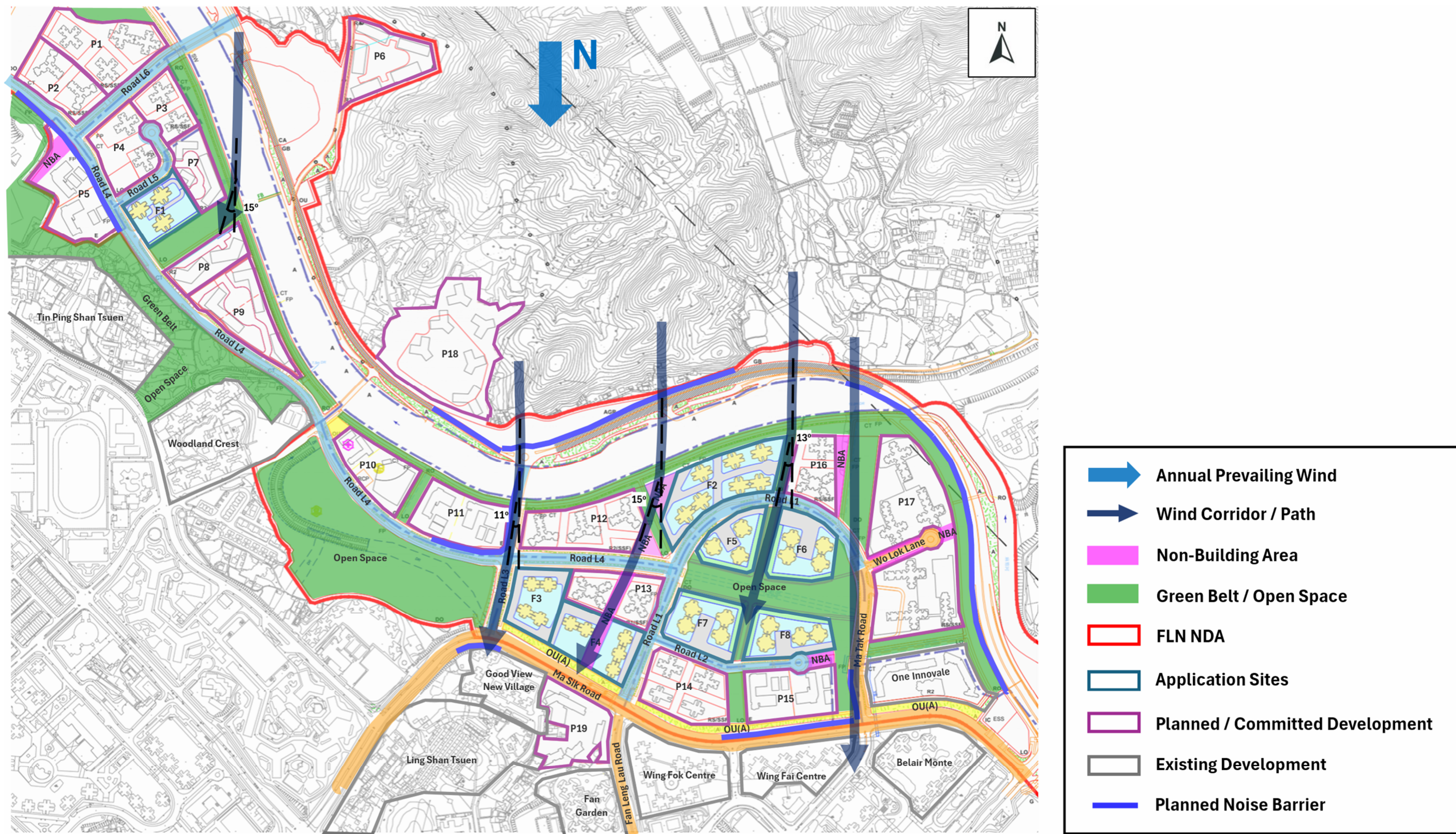
Figure 5.4-6 Wind Flow under the N Annual Prevailing Wind for the Proposed Scheme
