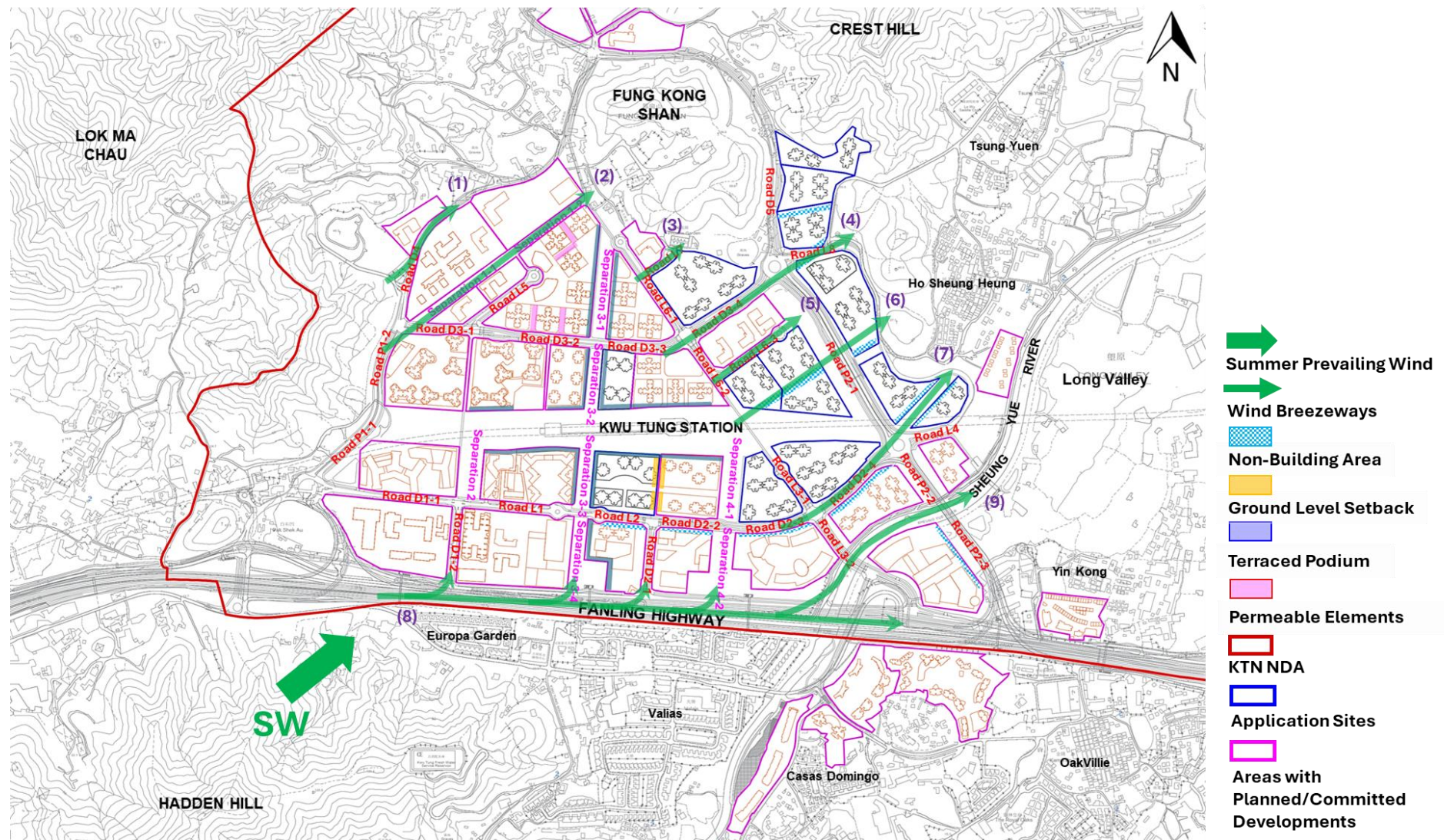
Figure 8.5(a) Wind Flow under the SW Summer Prevailing Wind for the Approved Scheme
