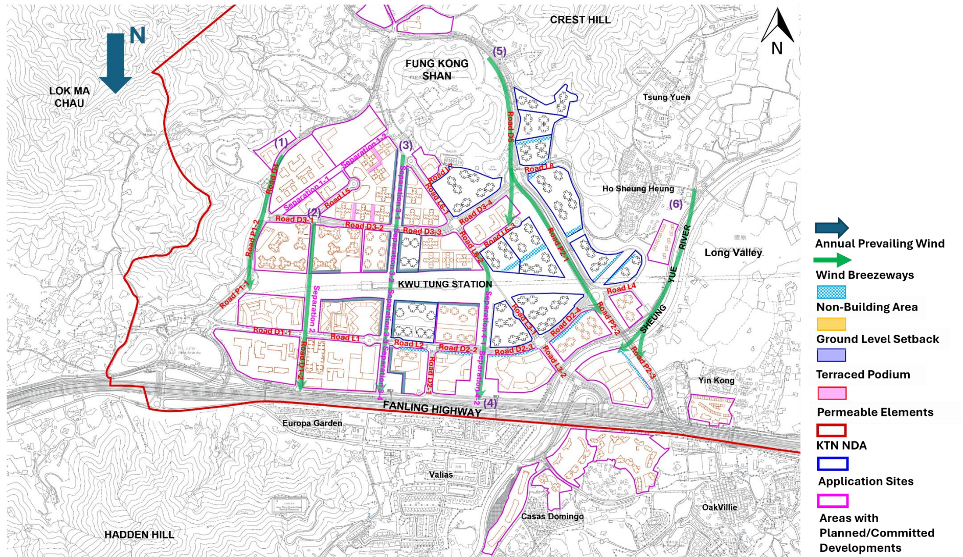
Figure C2.1(a) Wind Flow under the N Annual Prevailing Wind for the OZP Compliant Scheme
