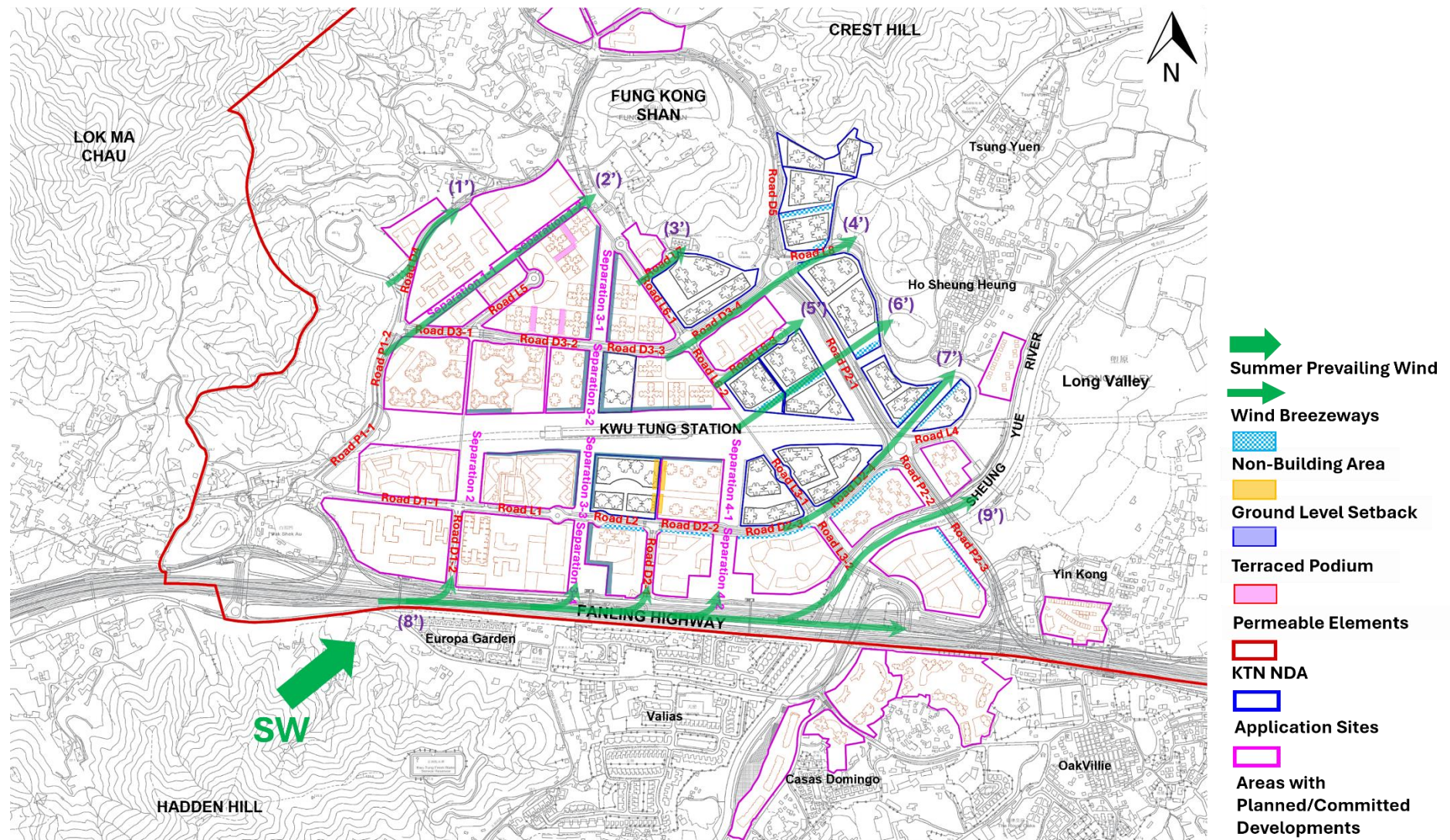
Figure 8.5(b) Wind Flow under the SW Summer Prevailing Wind for the Proposed Scheme
