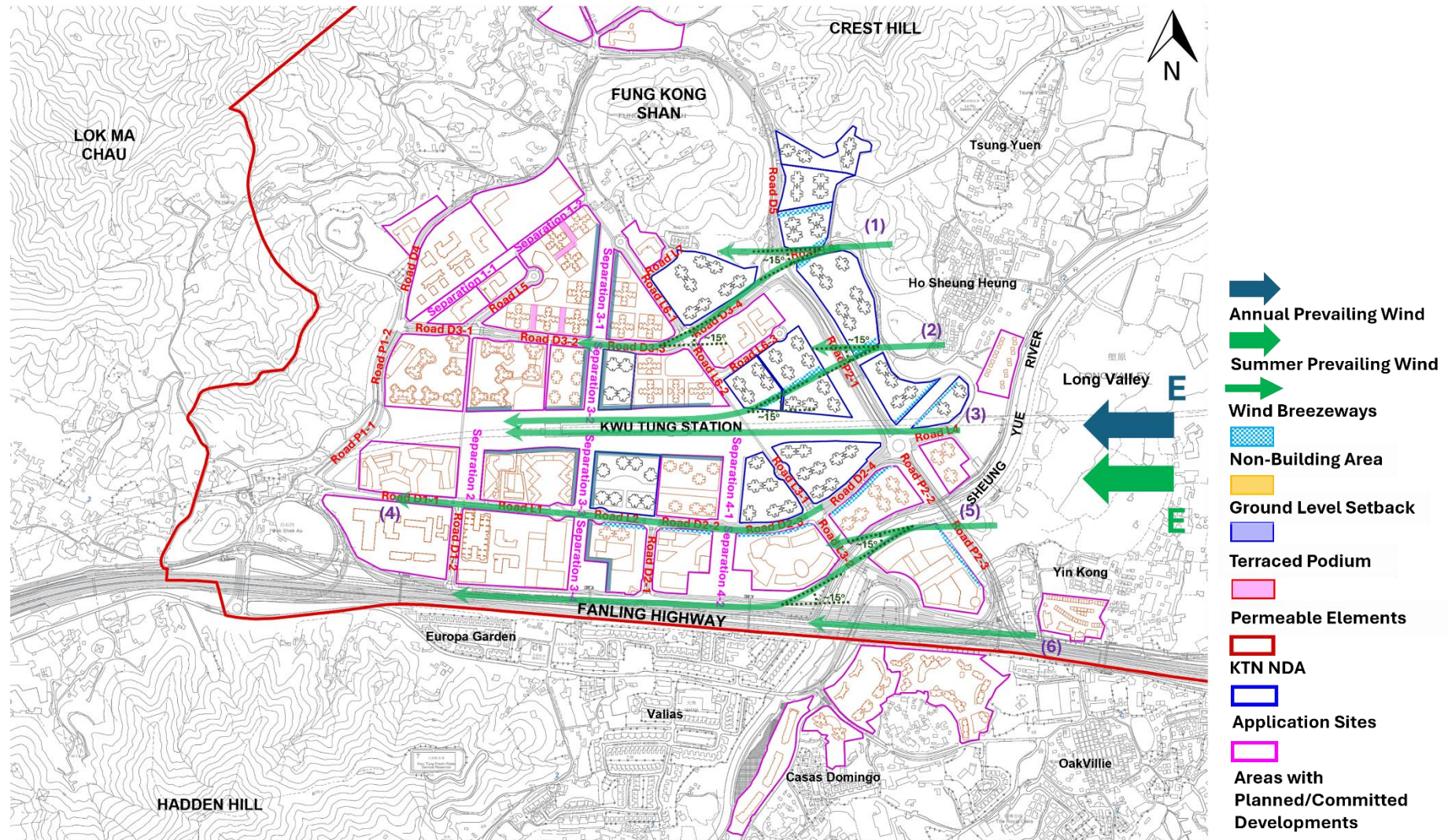
Figure C2.3(a) Wind Flow under the E Annual and Summer Prevailing Wind for the OZP Compliant Scheme
