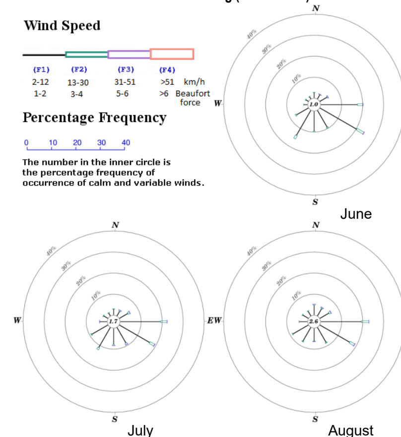
Figure 3.1-3 Summer Wind Rose from Ta Kwu Ling Weather Station Jun – Aug (1986 – 2024)
