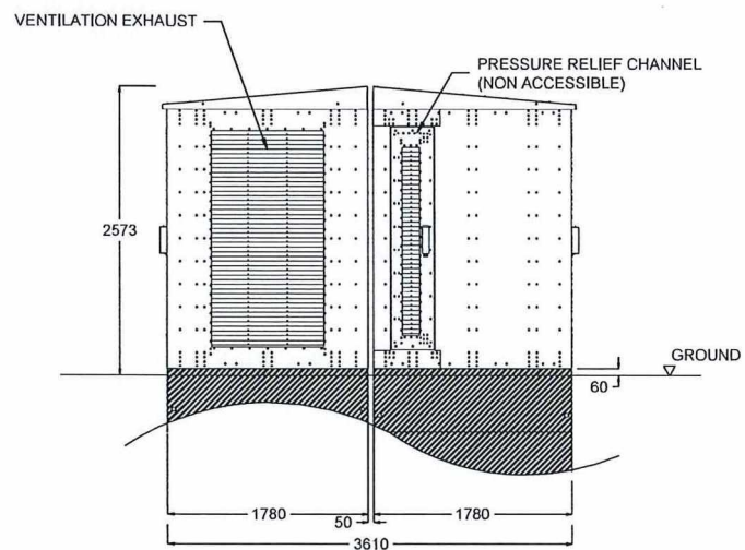
LEFT VIEW
