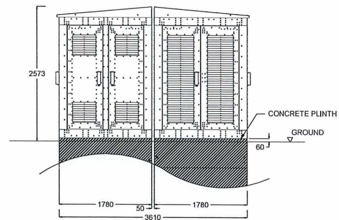
RIGHT VIEW
