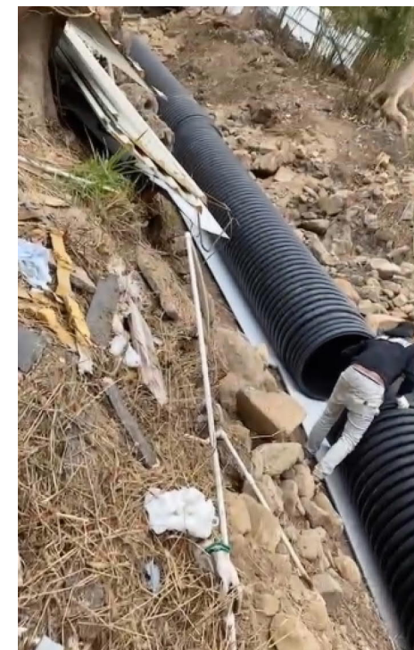
Site photo of typical ID900 corrugated HDPE pipe
