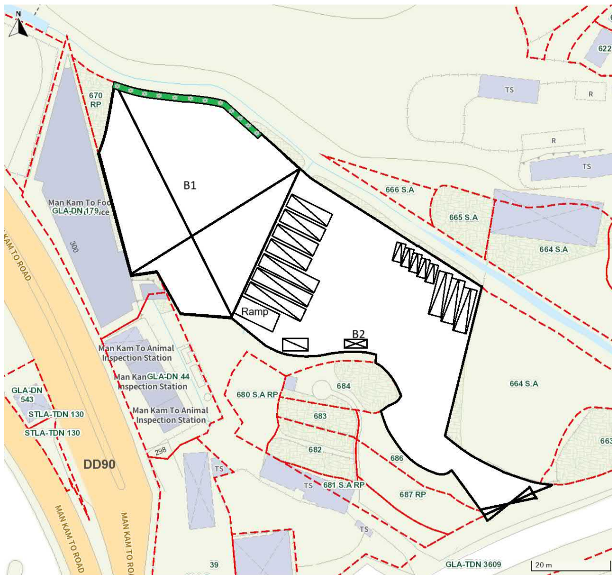
Figure 2 Revised Site Layout (Ingress/Egress)
