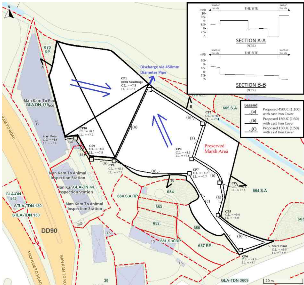
Figure 3 Revised Drainage Plan
