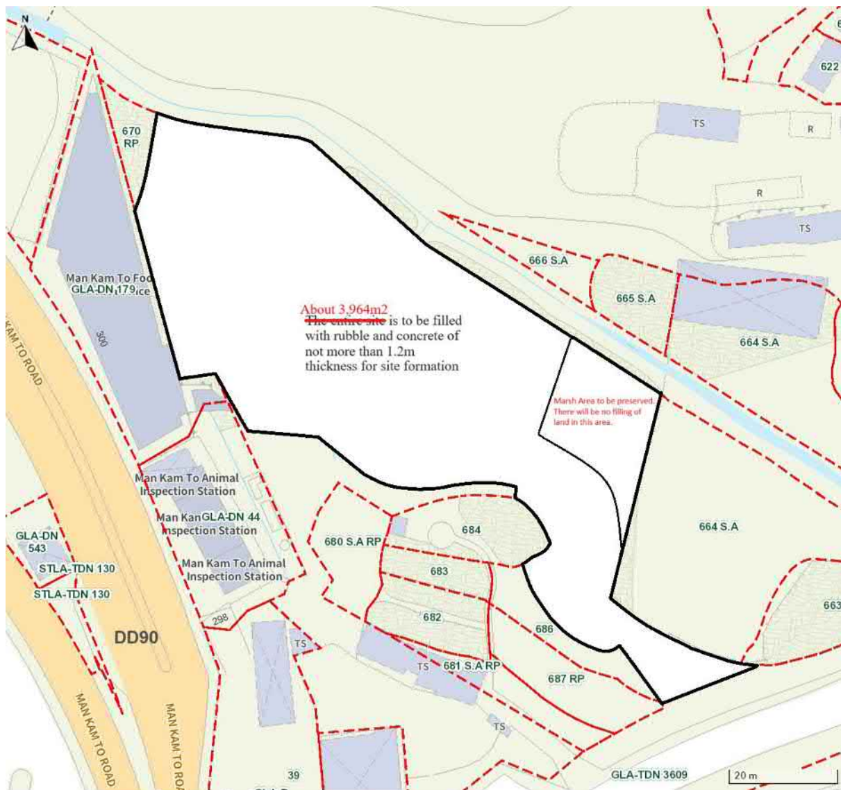
Figure 4 Revised Site Formation Plan
