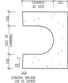
U-CHANNEL
