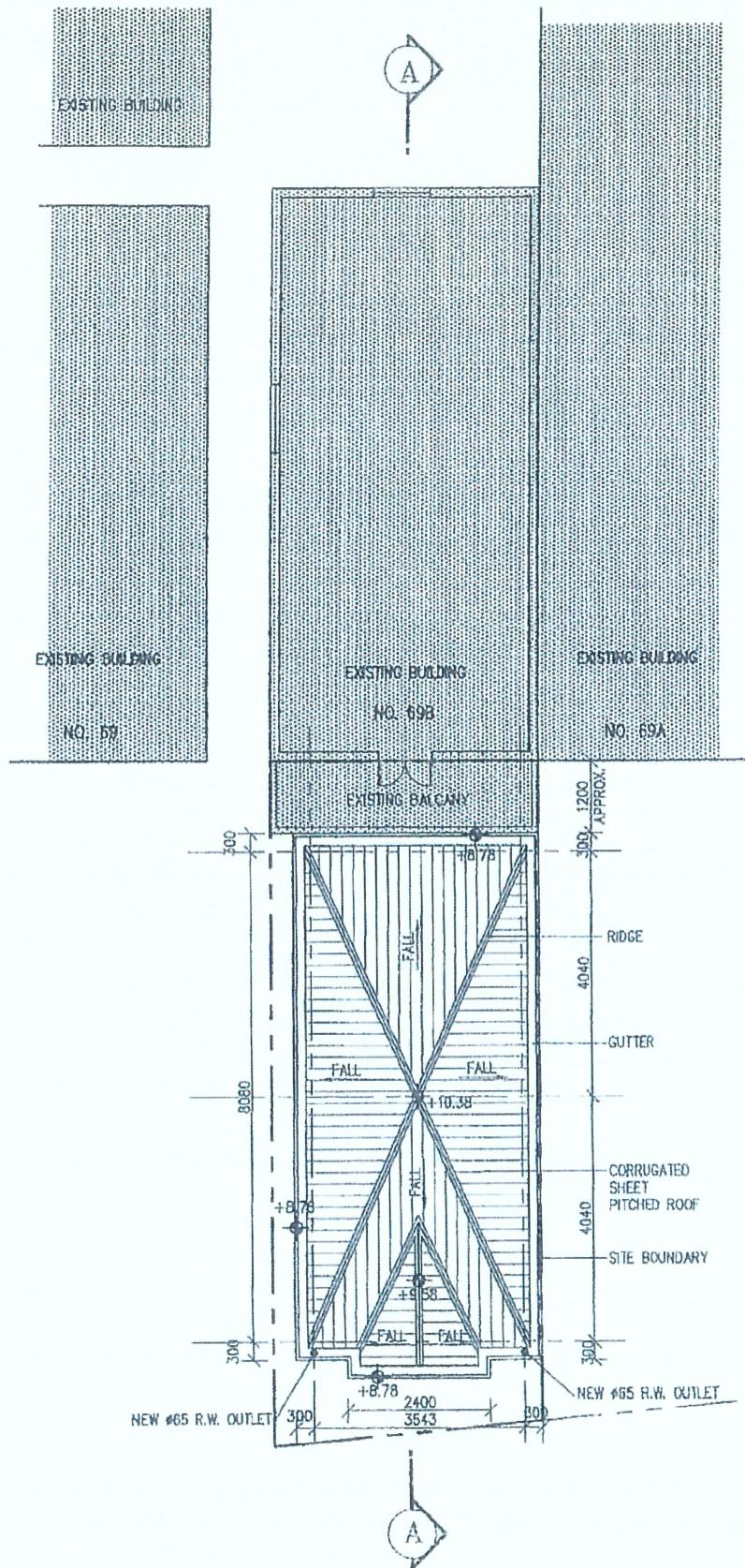
ROOF PLAN
