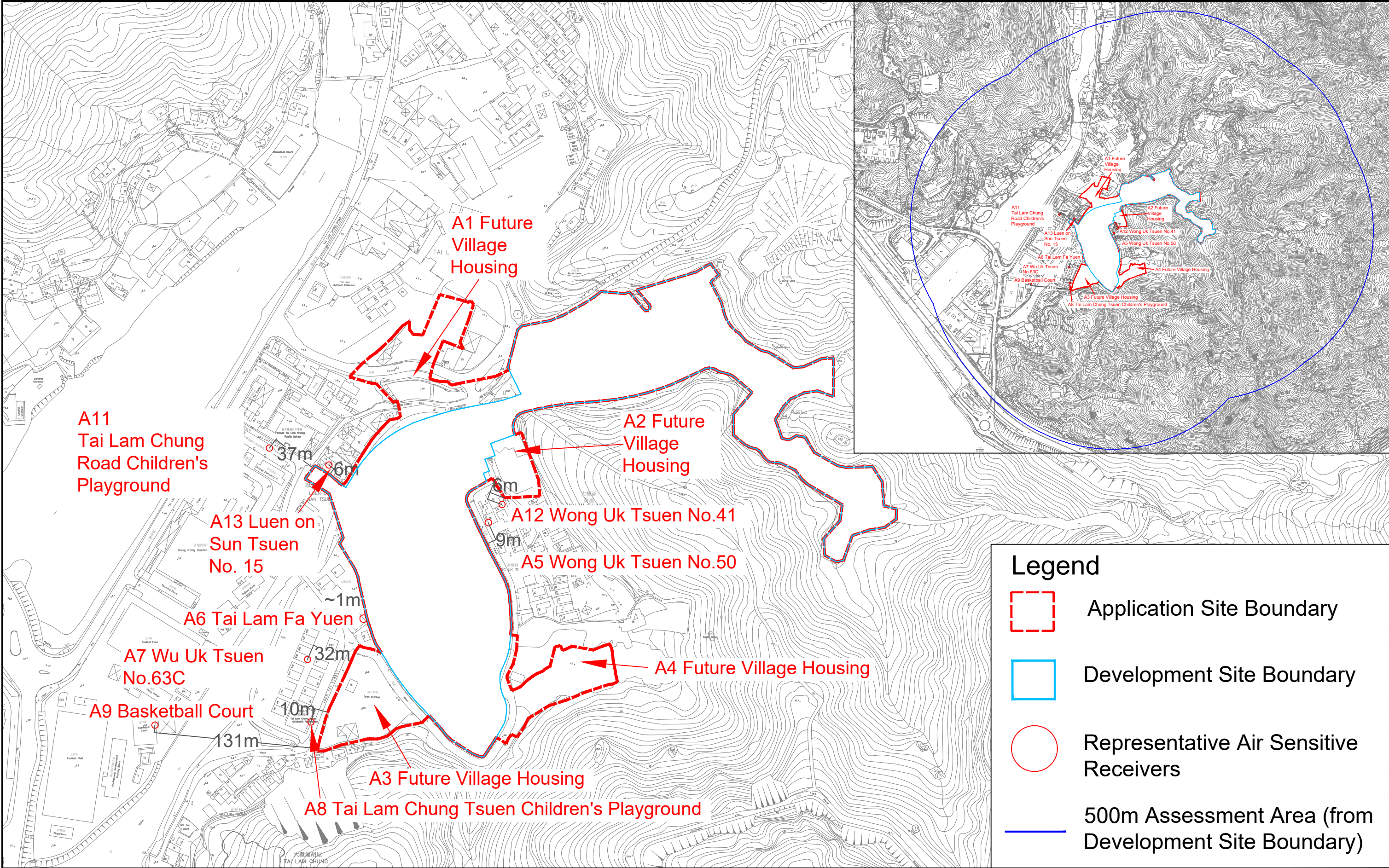
Figure: 4.6 Title: Location of Representative Air Sensitive Receivers During Construction Phase Drawn by: SC Project: Section 16 Planning Application for Proposed Amendments to a Comprehensive Residential Development Scheme (Previously Approved under Application No. A/TM-SKW/32-1) and Minor Relaxation of GFA and Building Height Restrictions at Various Lots in D.D. 385 and adjoining Government Land, Tai Lam Chung, Tuen Mun Checked by: TC Rev.: 1.0 Date: Sep 2024
