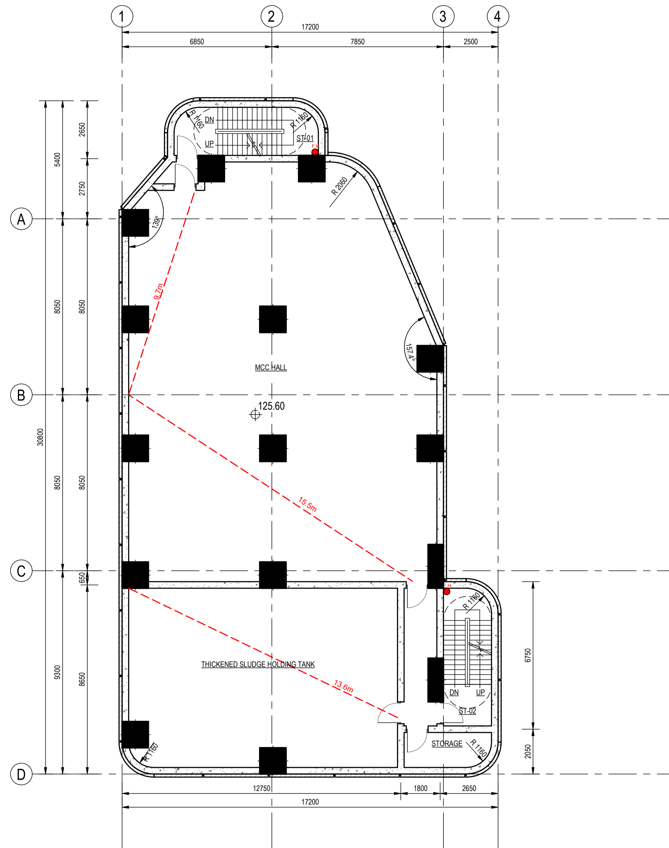
SECOND FLOOR SCALE 1 : 100
