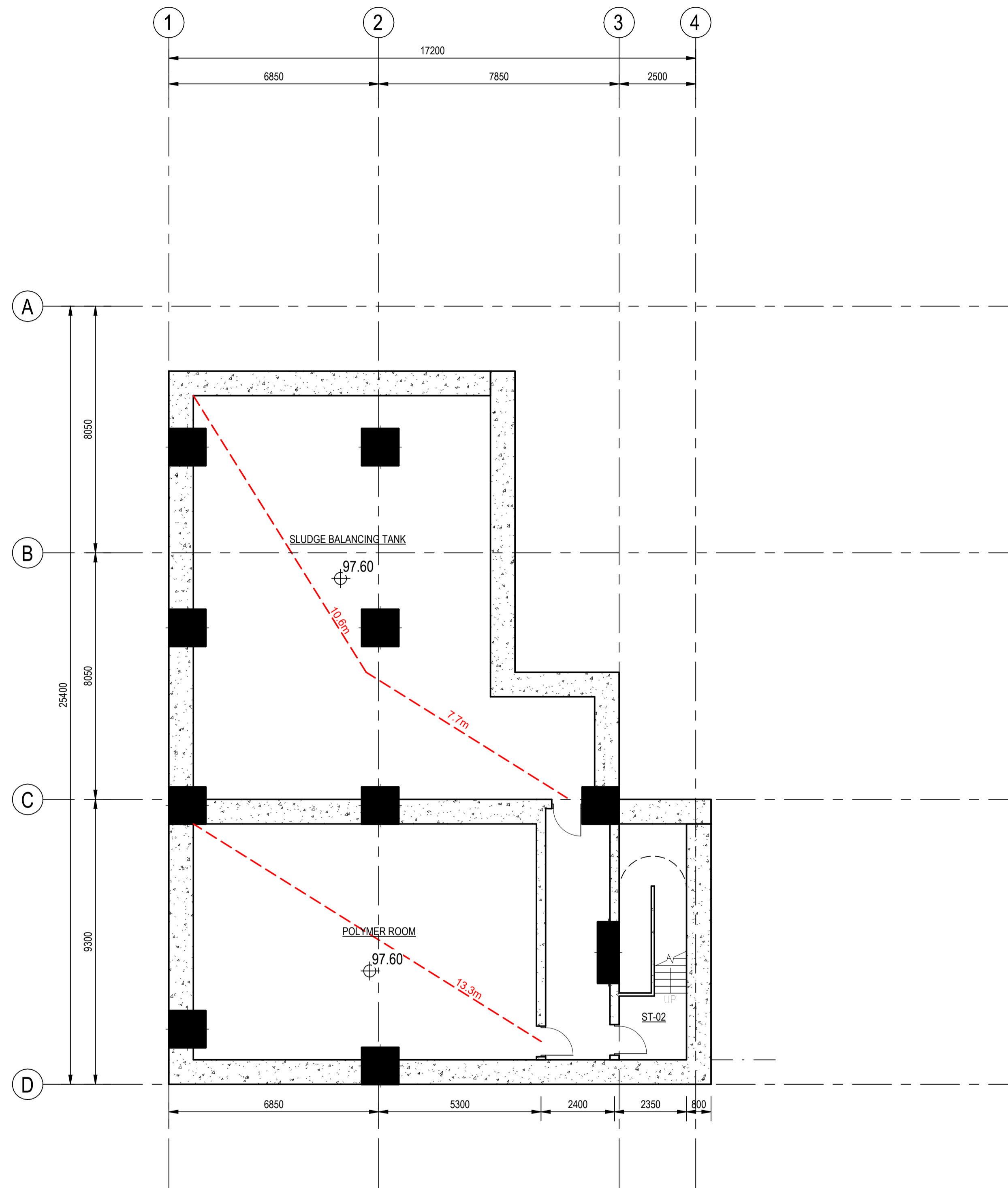
BASEMENT FLOOR SCALE 1 : 100
