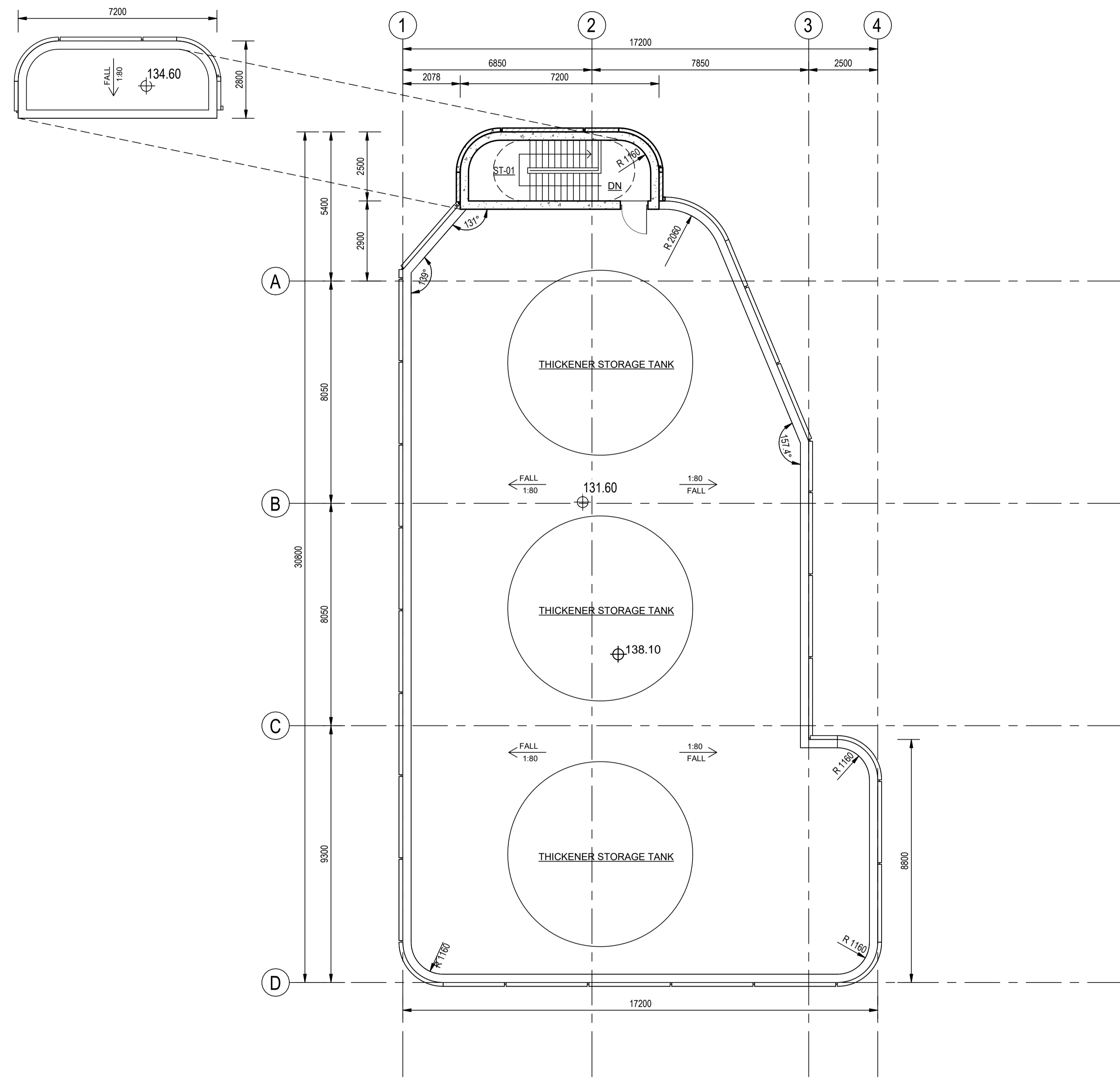
ROOF FLOOR SCALE 1 : 100
