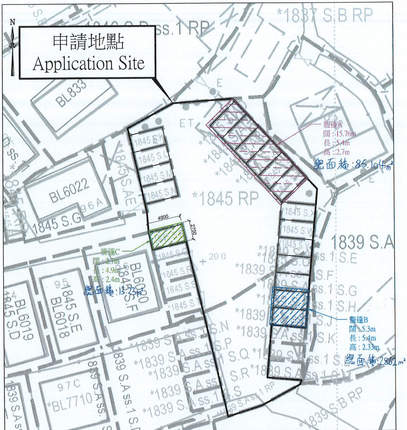
LAYOUT PLAN SHOWING CANOPY LOCATION AND DIMENSIONS (SCALE 1:400)
