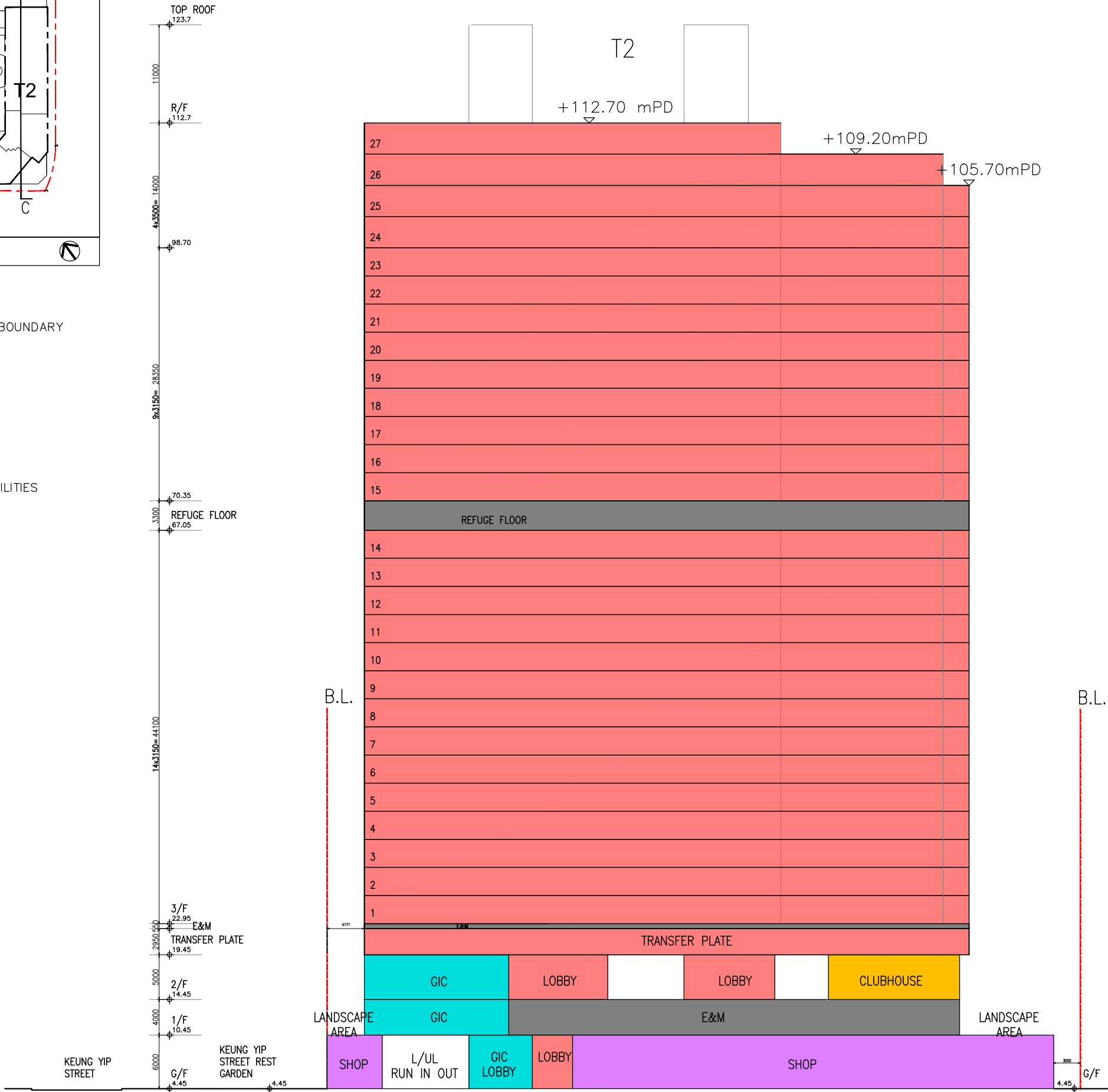
SECTION C-C
