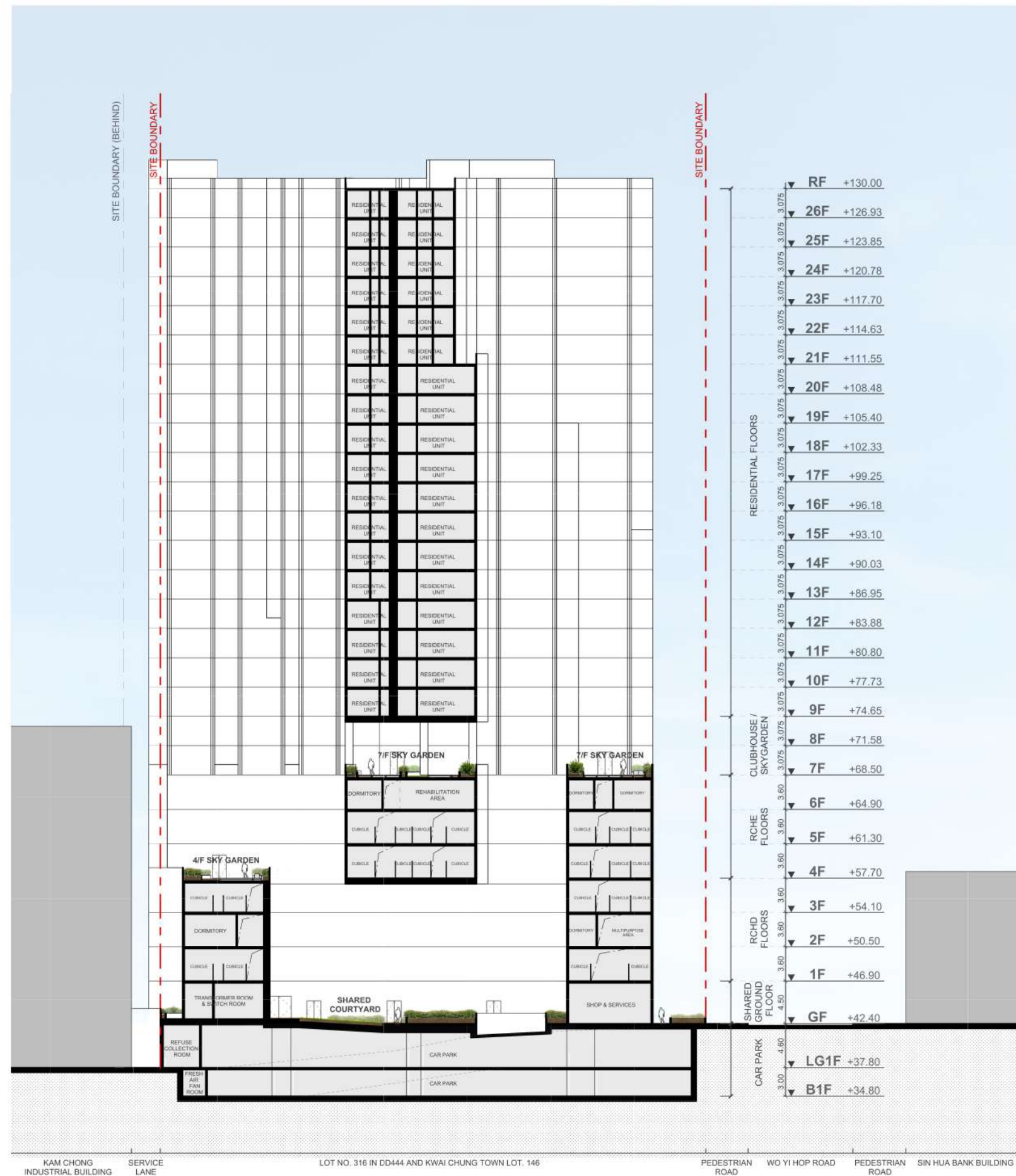
SCHEMATIC SECTION X-X'
