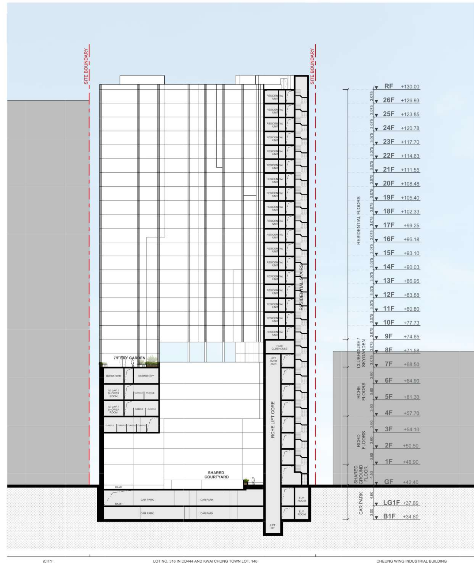
SCHEMATIC SECTION Y-Y'
