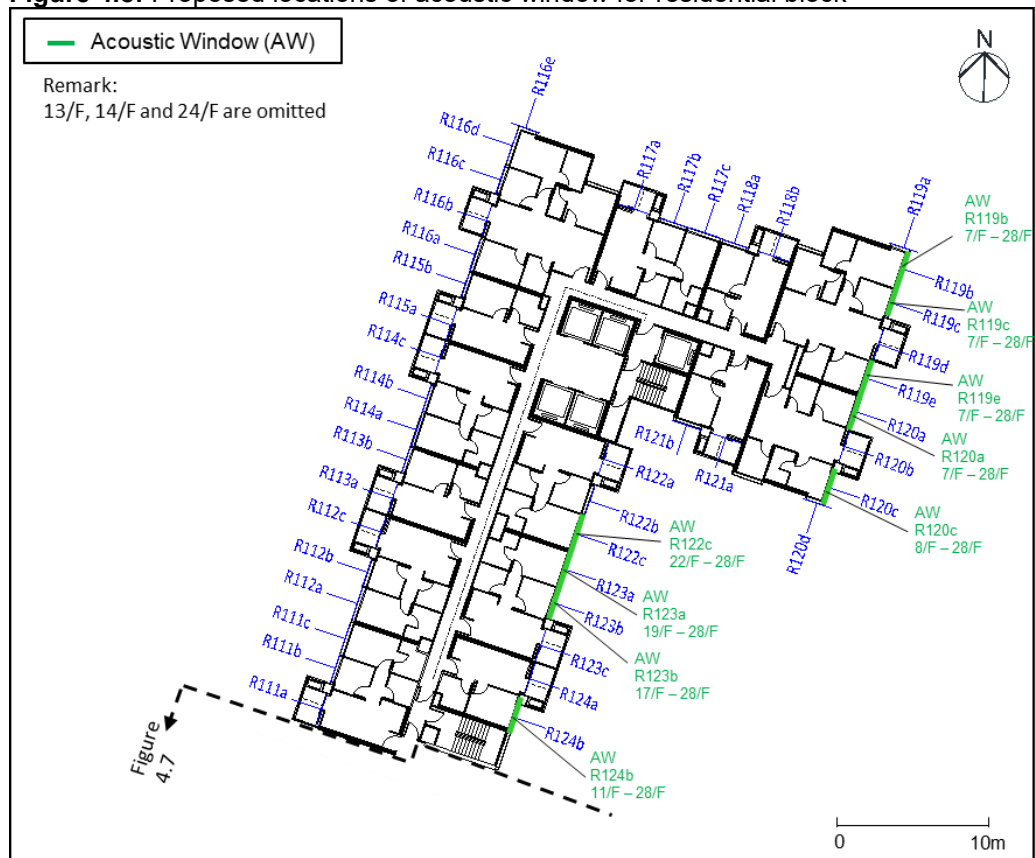
Figure 4.8: Proposed locations of acoustic window for residential block
