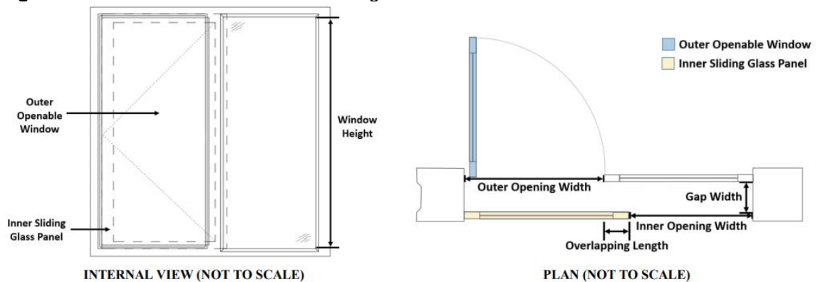
Figure 4.6: Schematic and sectional drawing of acoustic window
