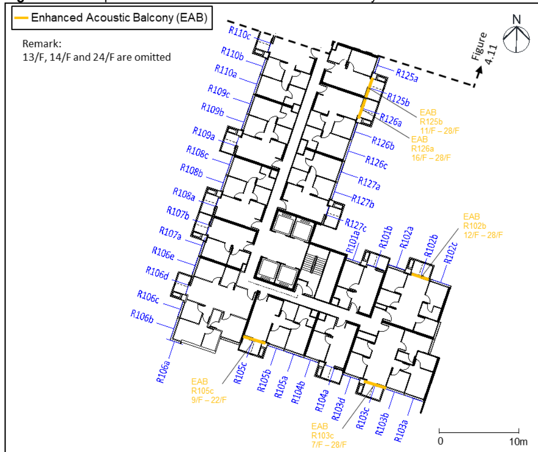
Figure 4.11: Proposed locations of enhanced acoustic balcony for residential block
