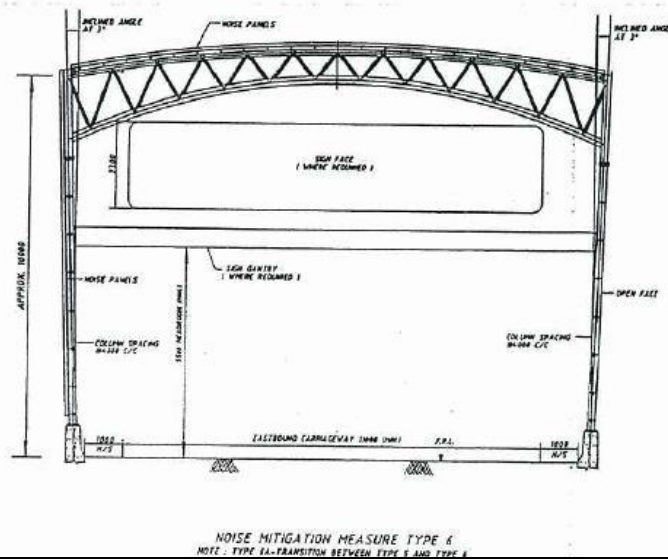
Project Title: Trunk Road T7 in Ma On Shan Figure 3: Noise Mitigation Measures Cross Sections
