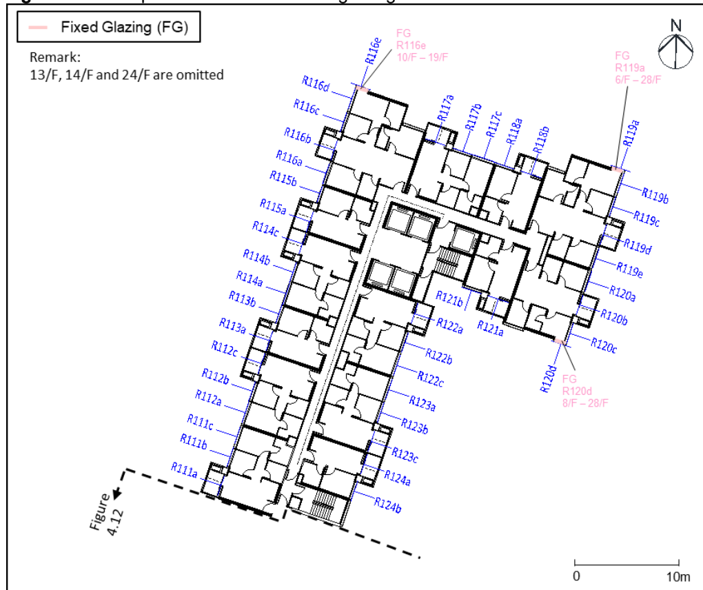
Figure 4.13: Proposed locations of fixed glazing for residential block
