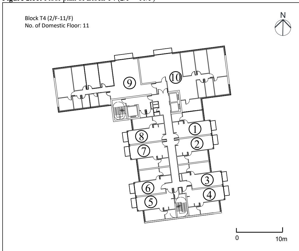
Figure 2.11: Floor plan of Block T4 (2/F – 11/F)
