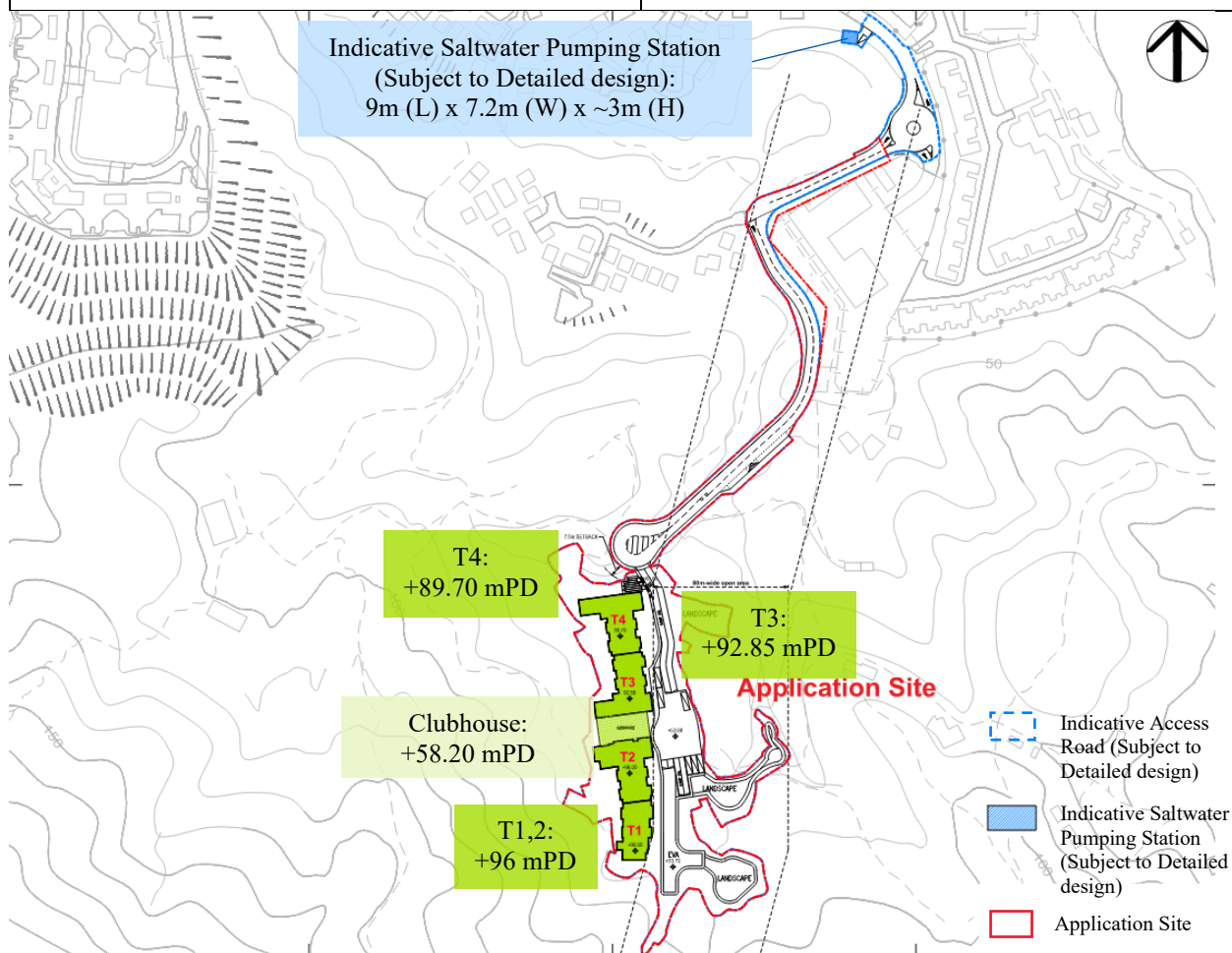
Figure 8 Master Layout Plan of Indicative Scheme
