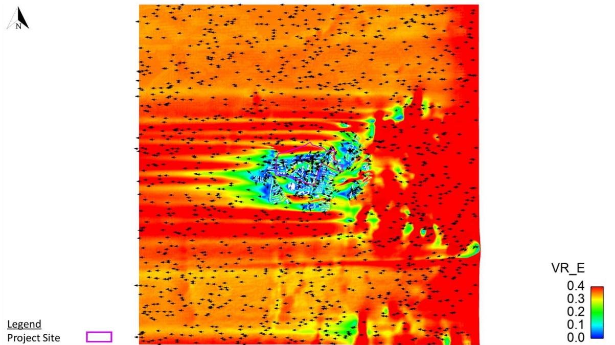
Figure 16 VR Vector Plot of Whole Domain at Pedestrian Level under E Wind for Proposed Scheme
