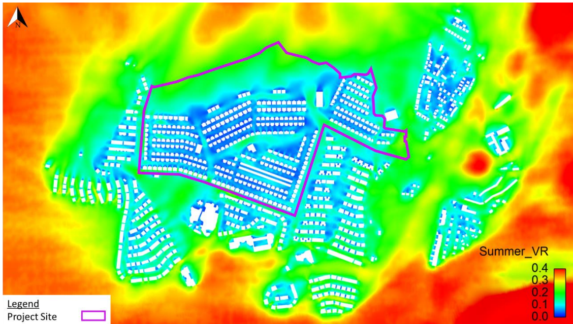
Figure 6.43: Summer Weighted Average VR Contour Plot at Pedestrian Level for Baseline Scheme
