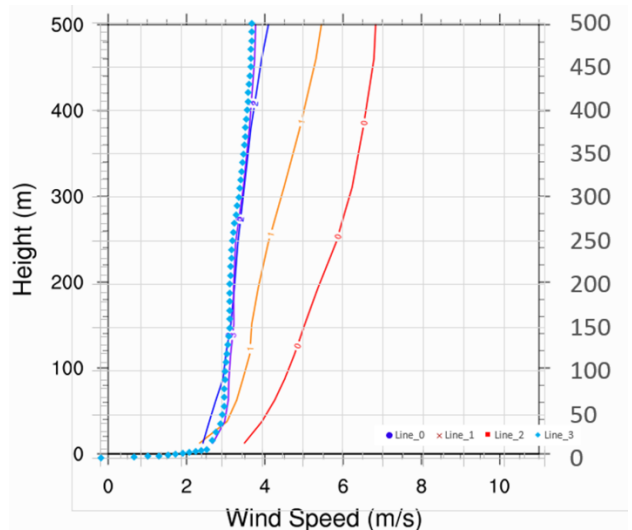
Figure 3.7: Wind Profile Curve for Wind Directions of 292.5° - 22.4° at Grid (X055, Y080)
