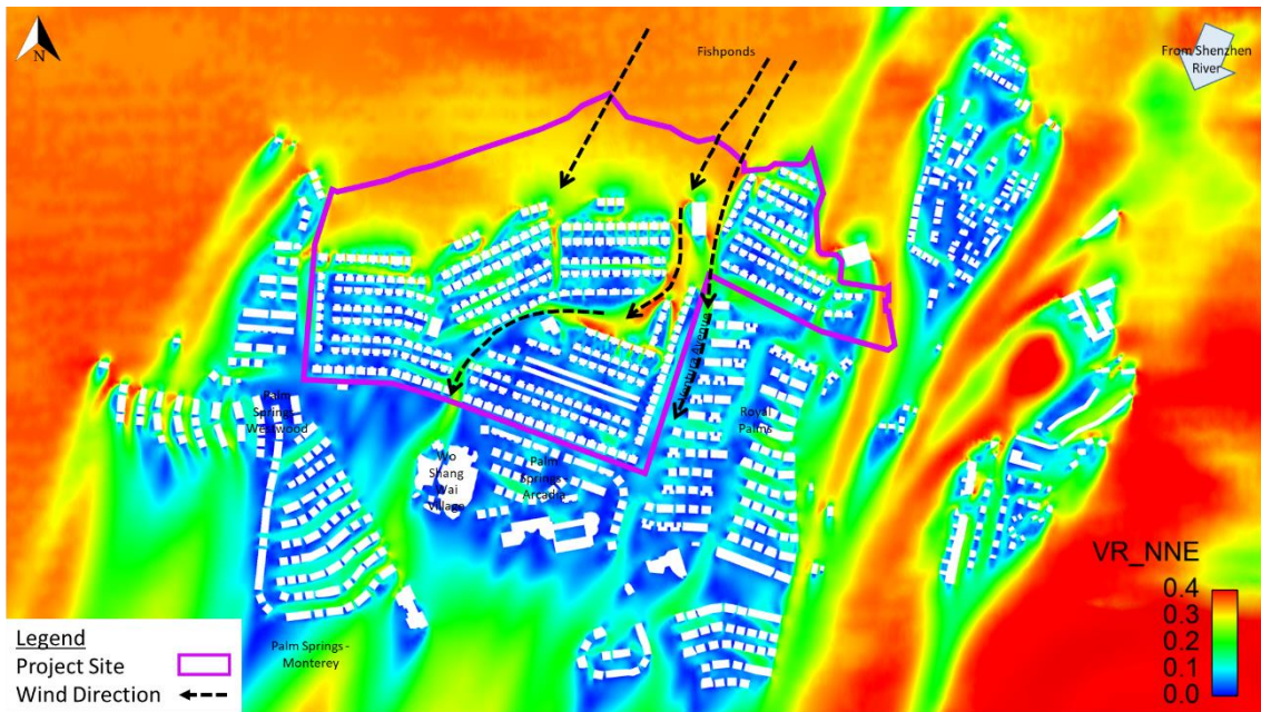
Figure 6.1: VR Contour Plot at Pedestrian Level under NNE Wind for Baseline Scheme
