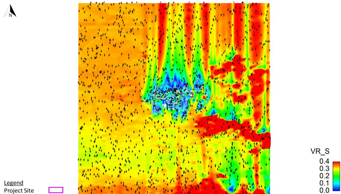
Figure 32 VR Vector Plot of Whole Domain at Pedestrian Level under S Wind for Proposed Scheme
