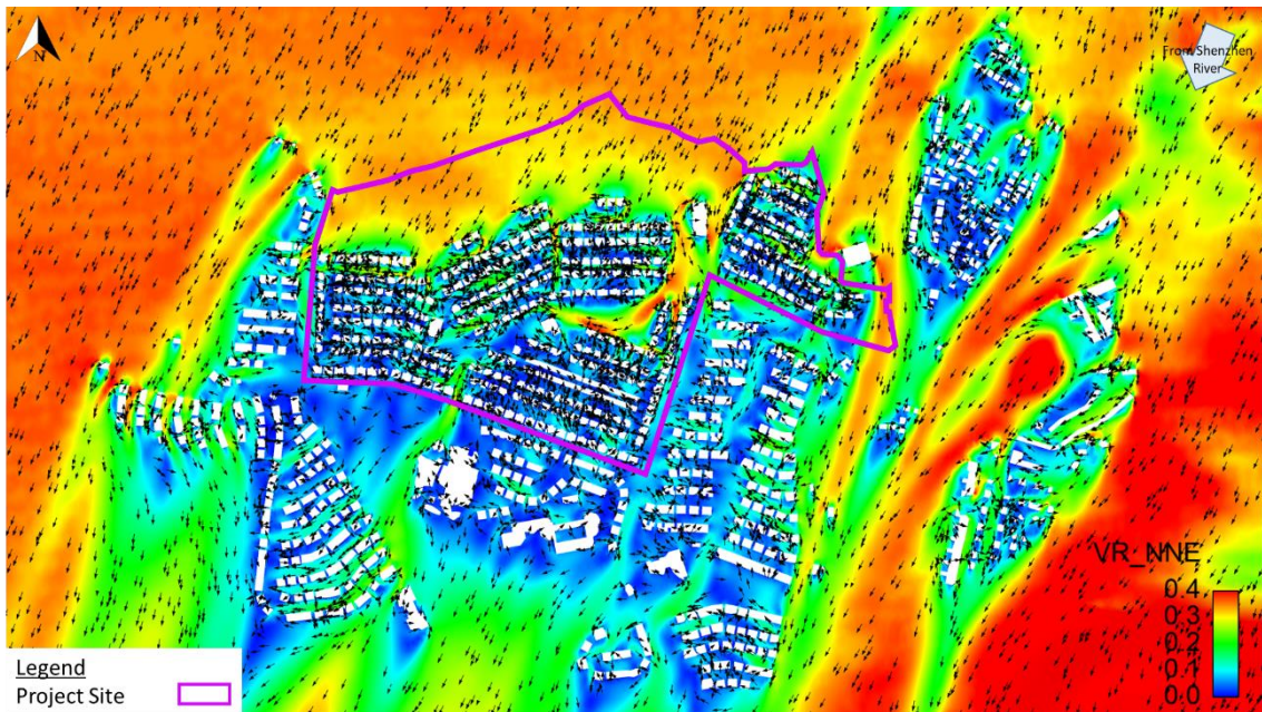
Figure 6.2: VR Vector Plot at Pedestrian Level under NNE Wind for Baseline Scheme
