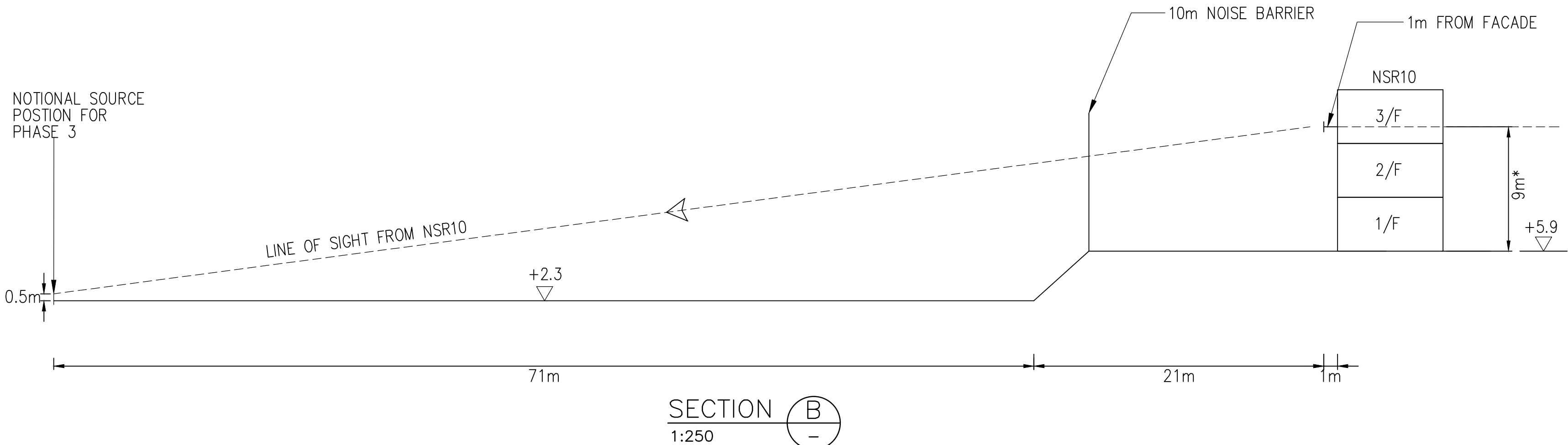
CROSS SECTION DIAGRAM SHOWING EXISTING TEMPORARY NOISE BARRIERS FOR CONSTRUCTION PHASE
