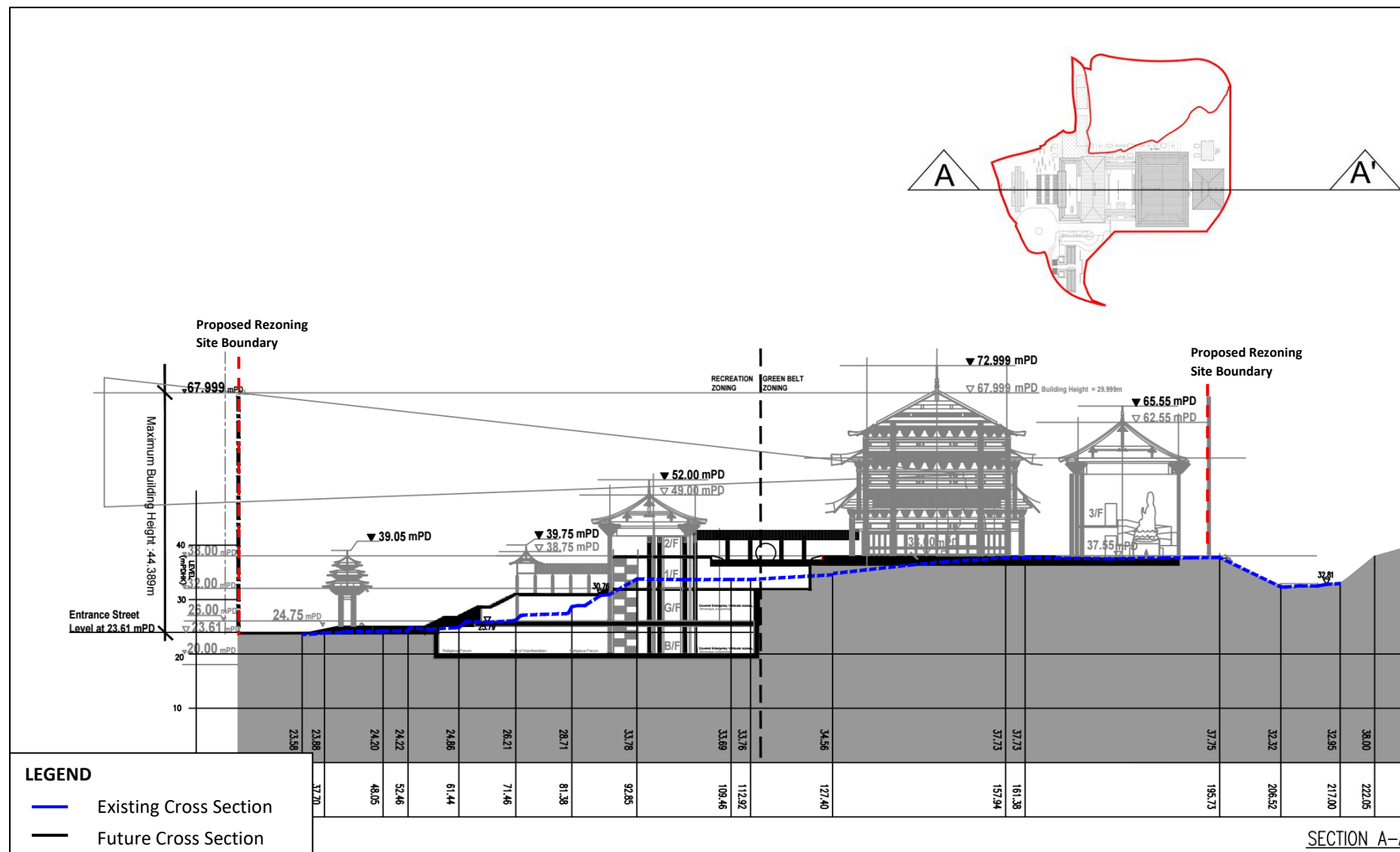
Figure C-1 Cross Sections of the Site (A-A 1 )
