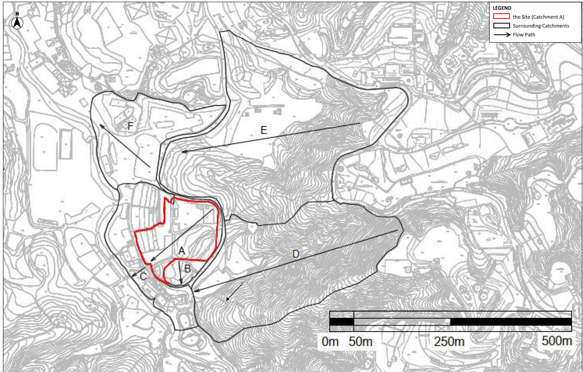
Figure 3-1 Identification of Catchments
