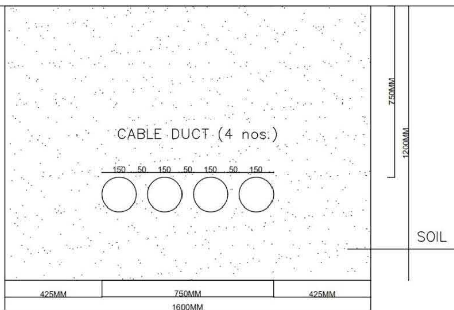
INDICATIVE SECTION OF UNDERGROUND CABLE TRENCH
