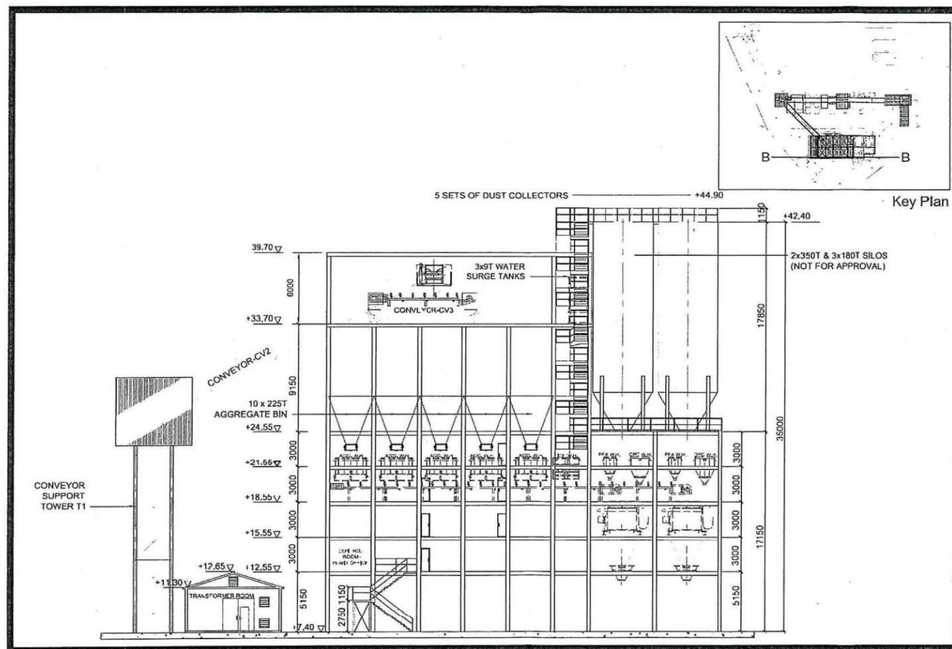
Section Plan B – B
