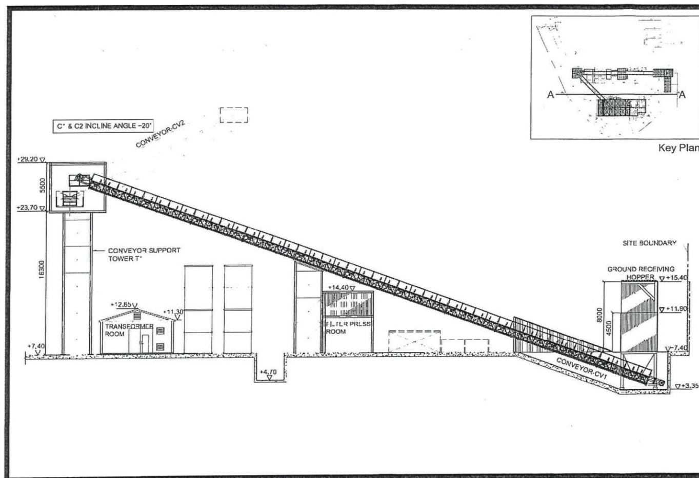
Section Plan A – A
