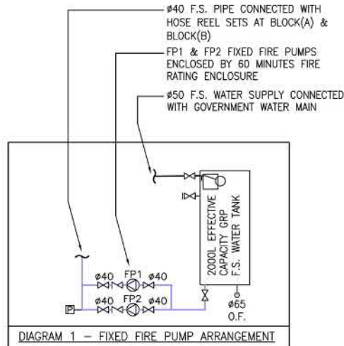
DIAGRAM 1 - FIXED FIRE PUMP ARRANGEMENT
