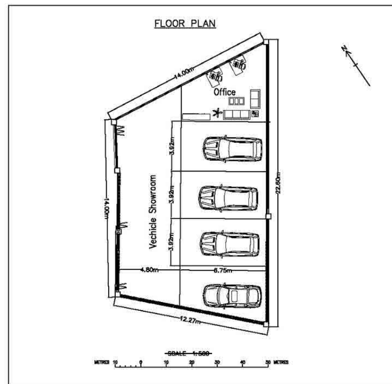
Figure 4A Indicative Layout Plan and Elevation
